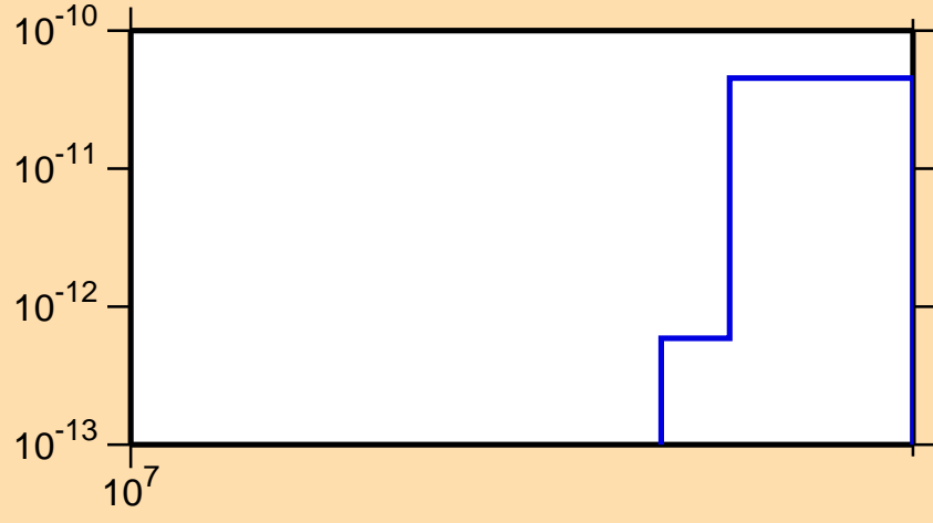
\sigma vs. E for ^{179}\text{Ir}(n,\text{pt})
