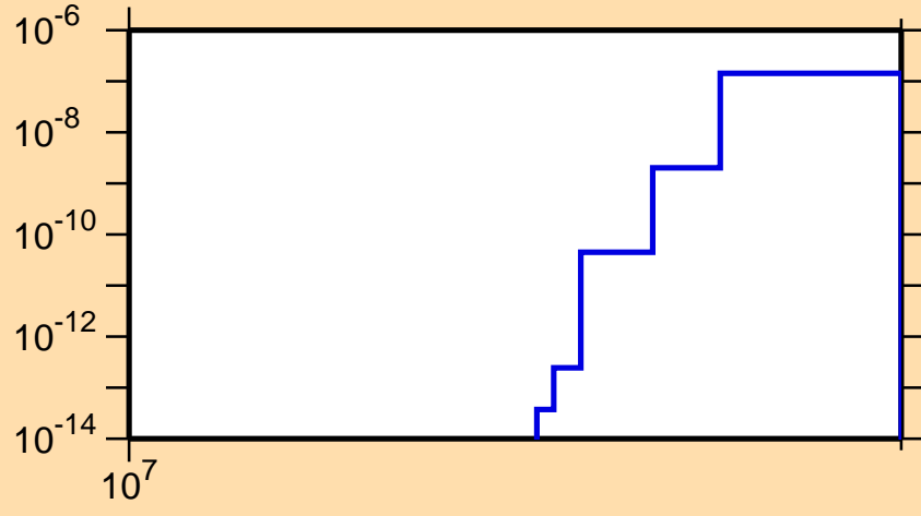
\sigma vs. E for ^{179}\text{Ir}(n,nt)
