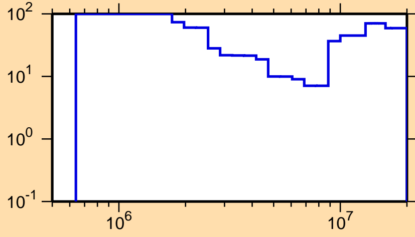
\Delta\sigma/\sigma vs. E for ^{179}\text{Ir}(n,n\text{cont.})
