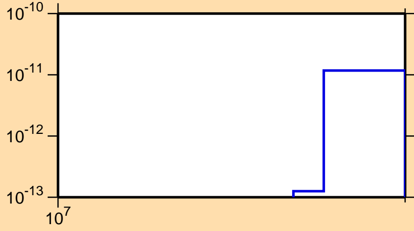
\sigma vs. E for ^{179}\text{Ir} (mt 34)
