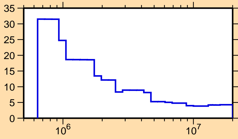
\Delta\sigma/\sigma vs. E for ^{179}\text{Ir}(n,\text{nonel.})
