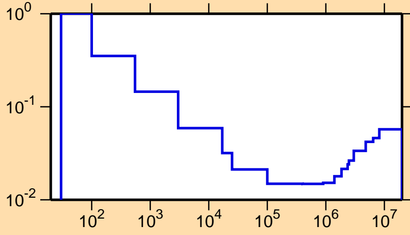
\sigma vs. E for ^{179}\text{Ir}(n,p)
