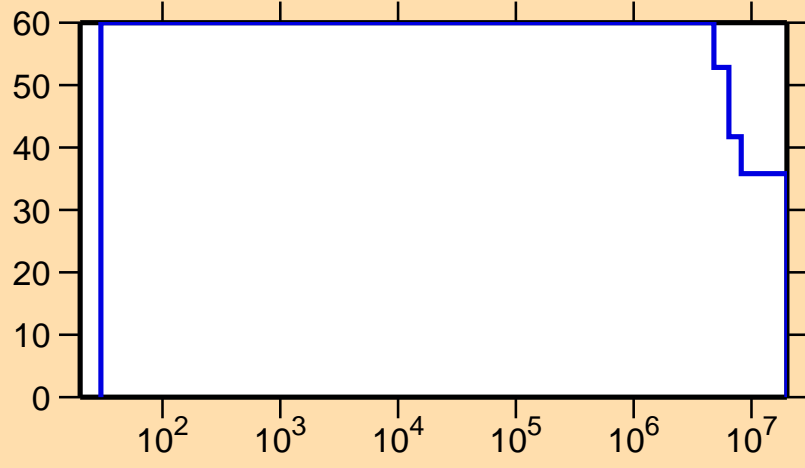
\Delta\sigma/\sigma vs. E for ^{179}\text{Ir}(n,p)
