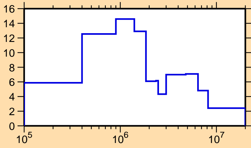
\Delta\sigma/\sigma vs. E for ^{179}\text{Ir}(n,\text{tot.})
