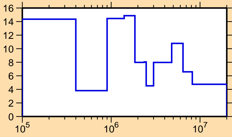
\Delta\sigma/\sigma vs. E for ^{179}\text{Ir}(n,\text{el.})
