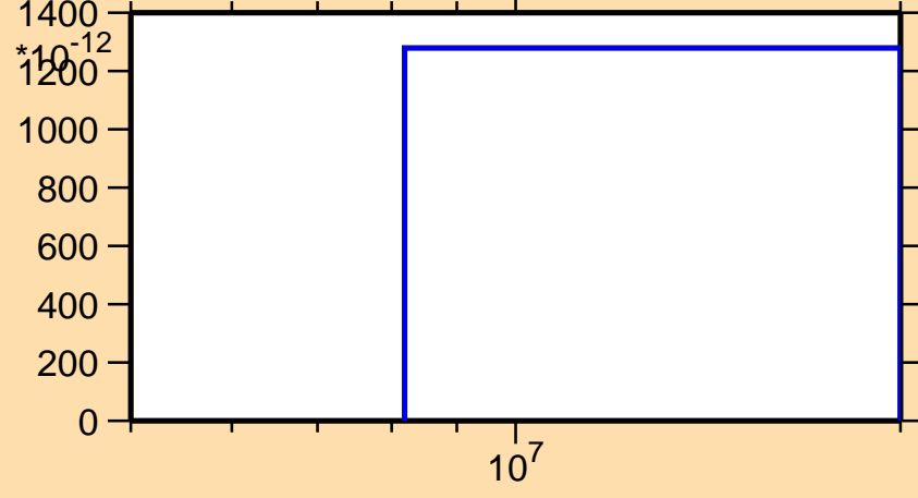
\sigma vs. E for ^{179}\text{Ir}(n,\text{pd})
