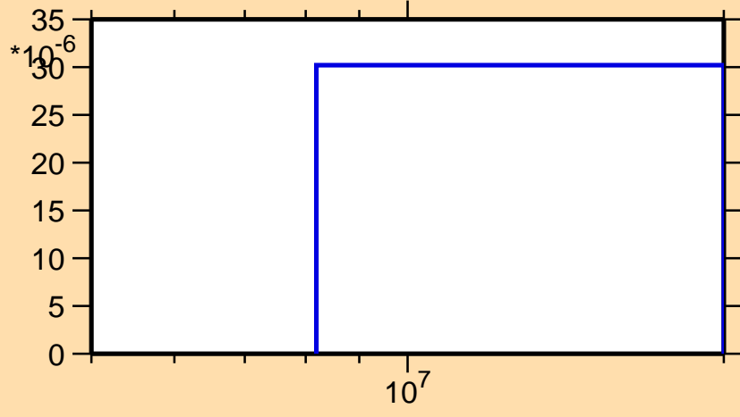
\sigma vs. E for ^{179}\text{Ir}(n,2np)
