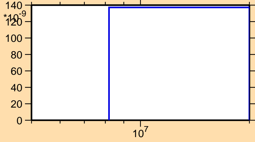
\sigma vs. E for ^{179}\text{Ir}(n,\text{nd})
