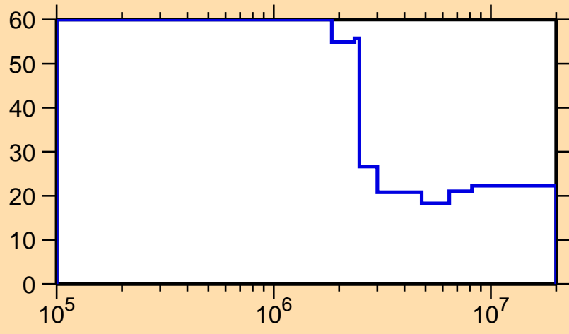
\Delta\sigma/\sigma vs. E for ^{179}\text{Ir}(n,n_1)
