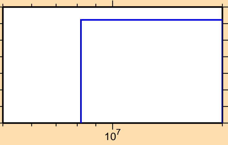
\sigma vs. E for ^{179}\text{Ir}(n,3n)
