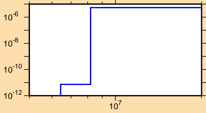
\sigma vs. E for ^{179}\text{Ir}(\text{mt } 45)
