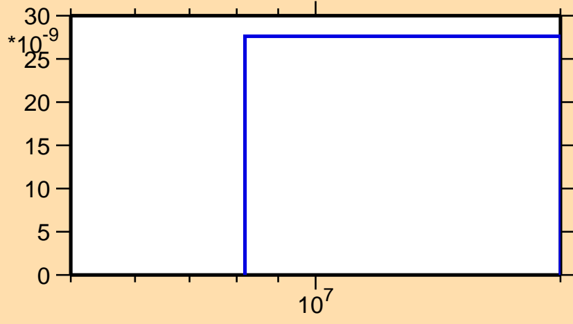
\sigma vs. E for ^{179}\text{Ir}(n,3n\alpha)
