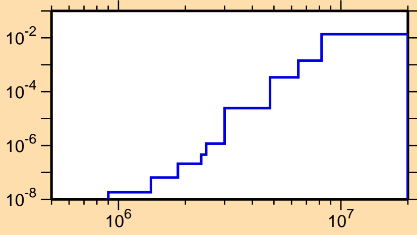
\sigma vs. E for ^{179}\text{Ir}(n,n\alpha)
