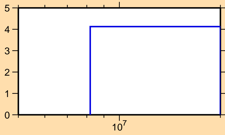
\Delta\sigma/\sigma vs. E for ^{179}\text{Ir}(n,\text{nonel.})
