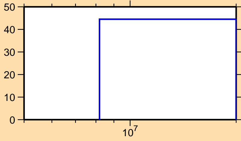
\Delta\sigma/\sigma vs. E for ^{179}\text{Ir}(n,2n)
