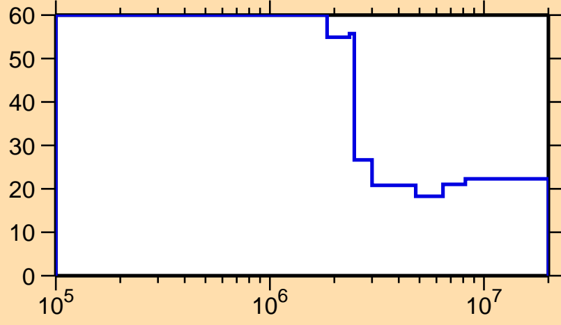
\Delta\sigma/\sigma vs. E for ^{179}\text{Ir}(n,n_1)
