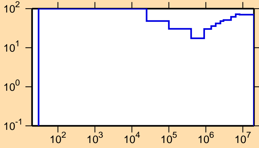
\Delta\sigma/\sigma vs. E for ^{179}\text{Ir}(n,\gamma)
