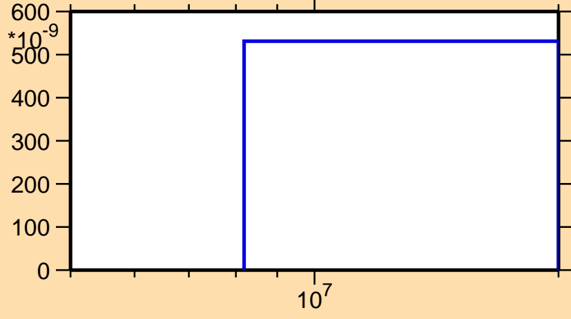
\sigma vs. E for ^{179}\text{Ir}(n,\text{He}3)
