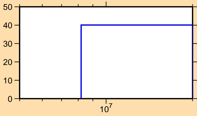
\Delta\sigma/\sigma vs. E for ^{179}\text{Ir}(n,\text{inel.})
