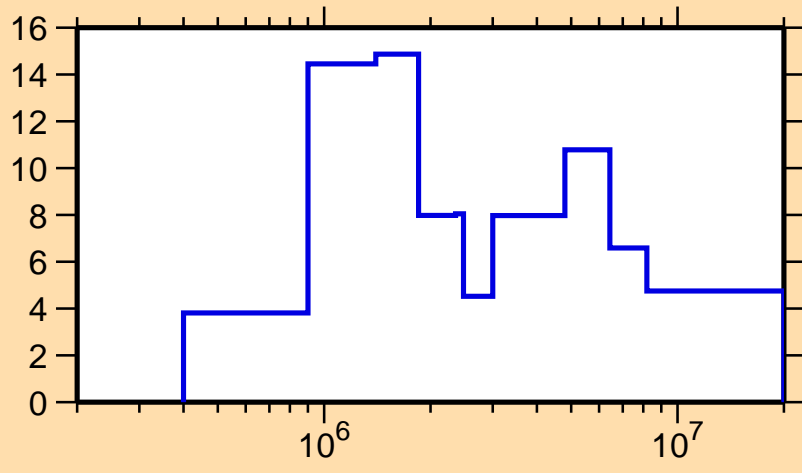
\Delta\sigma/\sigma vs. E for ^{179}\text{Ir}(n, el.)
