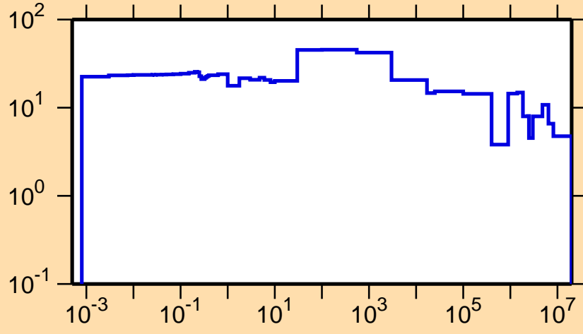
\Delta\sigma/\sigma vs. E for ^{179}\text{Ir}(n,\text{el.})
