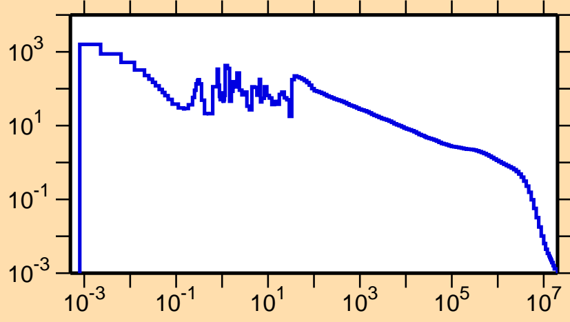
\sigma vs. E for ^{180}\text{Ir}(n,\gamma)
