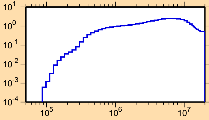
\sigma vs. E for ^{180}\text{Ir}(n,\text{inel.})
