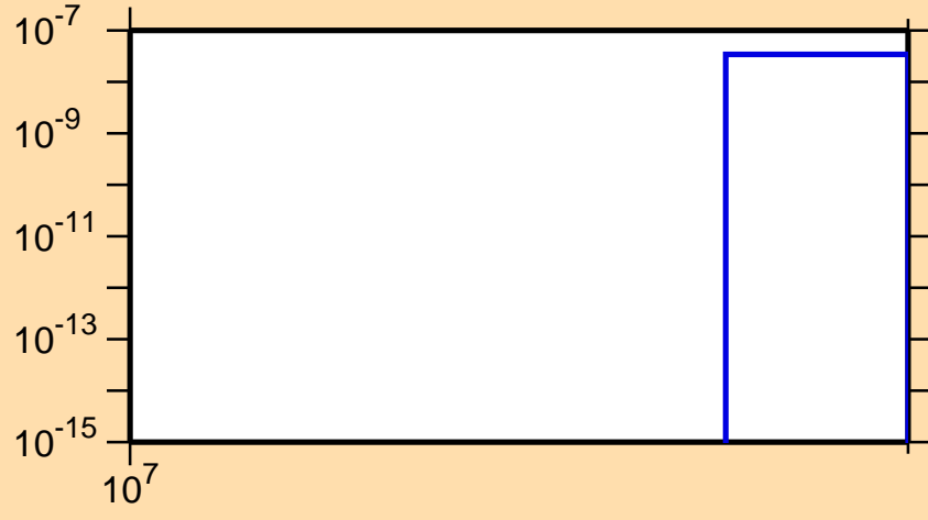
\sigma vs. E for ^{180}\text{Ir}(n,3n\alpha)
