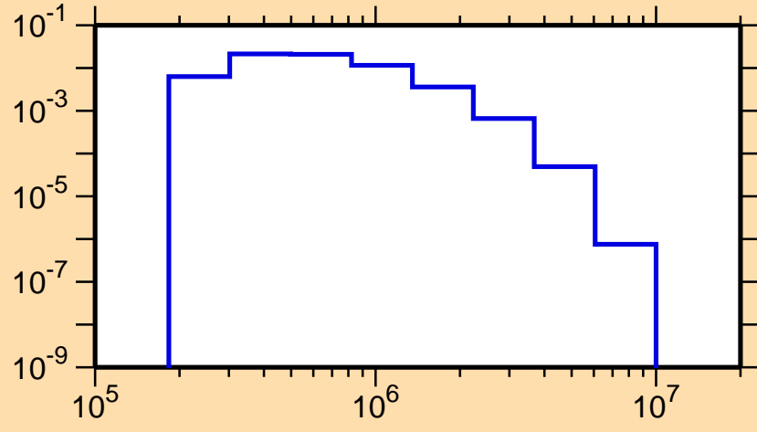
\sigma vs. E for ^{180}\text{Ir}(n,n_4)
