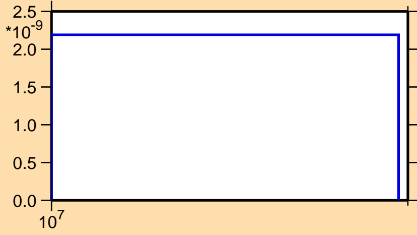
\sigma vs. E for ^{180}\text{Ir}(n,nt)
