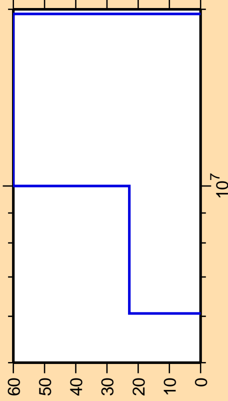
\Delta\sigma/\sigma vs. E for ^{180}\text{Ir}(n,n\text{cont.})
