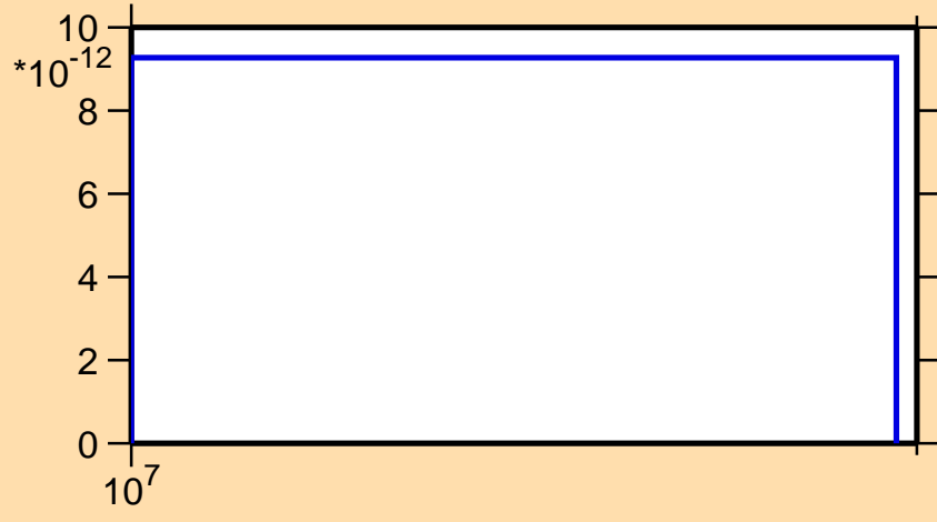
\sigma vs. E for ^{180}\text{Ir} (mt 34)
