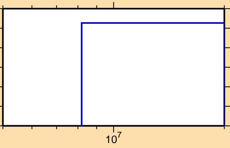
\sigma vs. E for ^{180}\text{Ir}(n,\text{pd})
