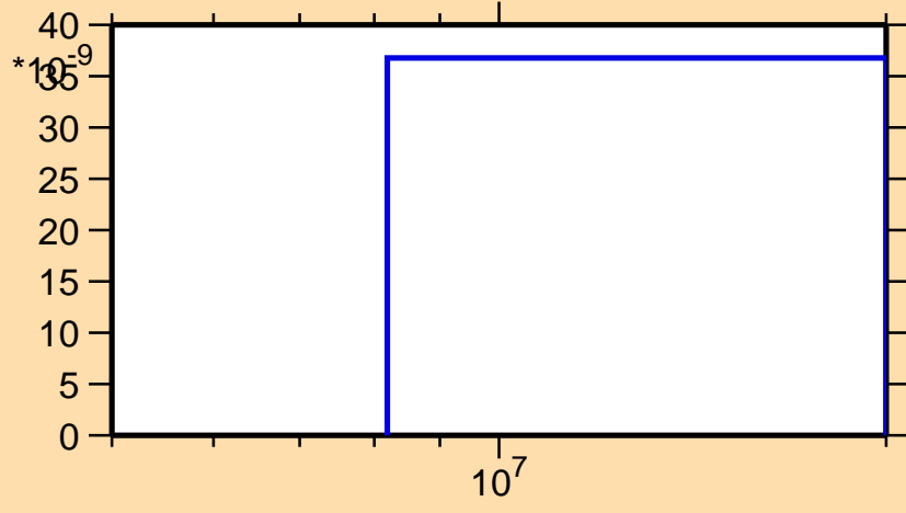
\sigma vs. E for ^{180}\text{Ir}(\text{mt117})
