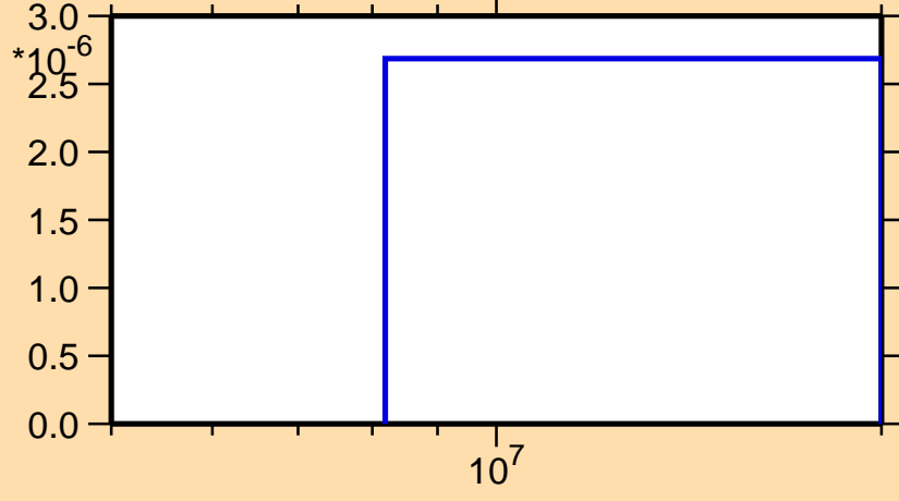
\sigma vs. E for ^{180}\text{Ir}(n,\text{nd})
