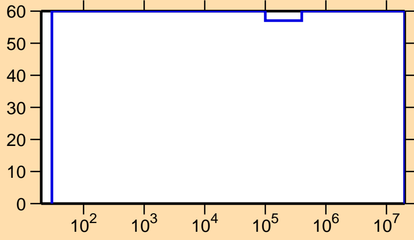
\Delta\sigma/\sigma vs. E for ^{180}\text{Ir}(n,\gamma)
