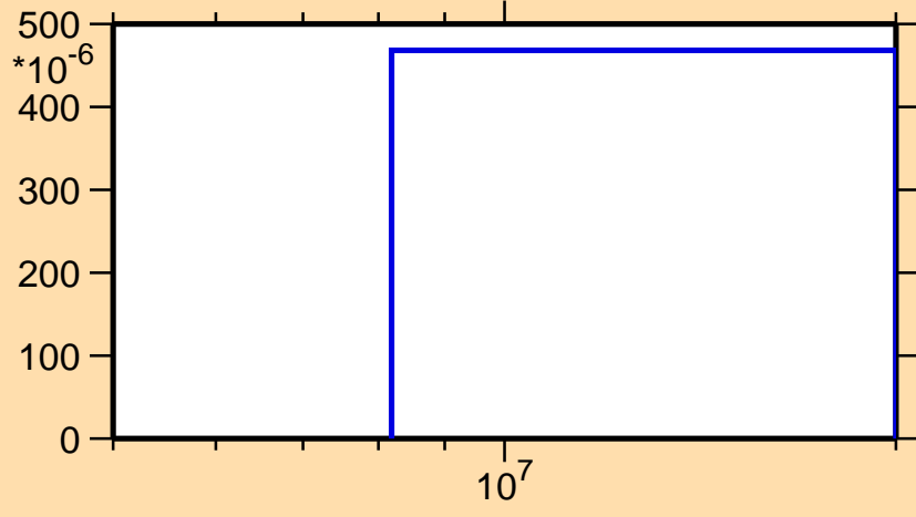
\sigma vs. E for ^{180}\text{Ir}(n,2np)
