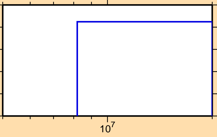
\sigma vs. E for ^{180}\text{Ir}(n,nt)
