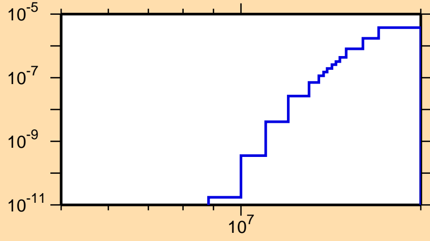
\sigma vs. E for ^{181}\text{Ir}(\text{mt } 45)
