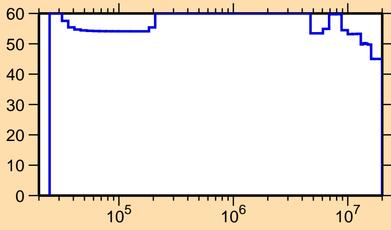
\Delta\sigma/\sigma vs. E for ^{181}\text{Ir}(n,n_1)
