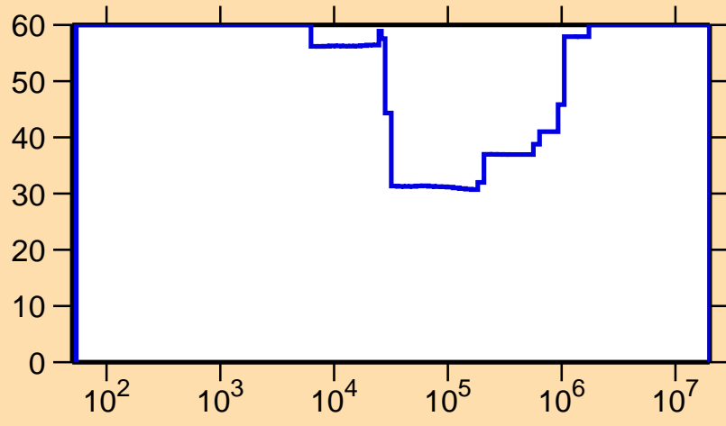
\Delta\sigma/\sigma vs. E for ^{181}\text{Ir}(n,\gamma)
