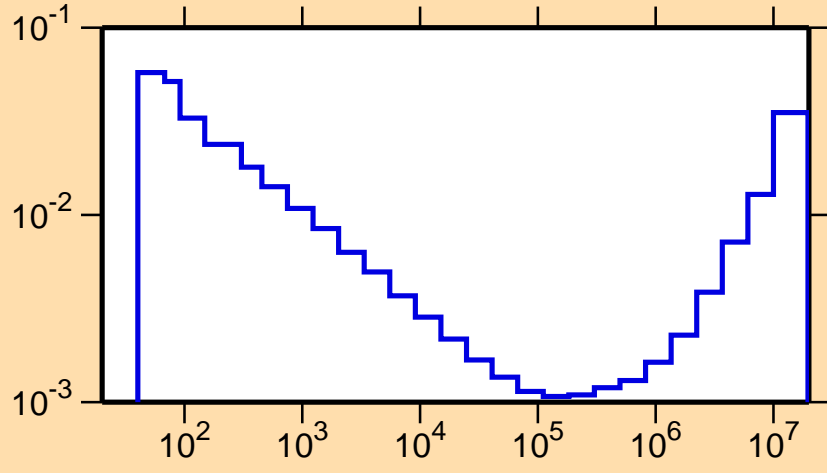
\sigma vs. E for ^{181}\text{Ir}(n,p)
