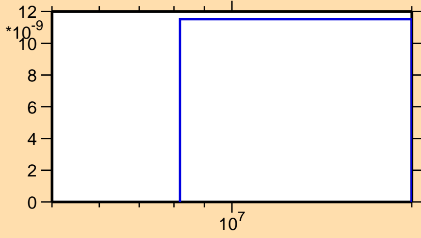
\sigma vs. E for ^{181}\text{Ir}(\text{mt117})
