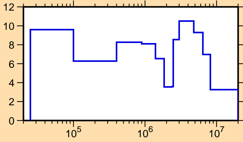
\Delta\sigma/\sigma vs. E for ^{181}\text{Ir}(n,\text{tot.})
