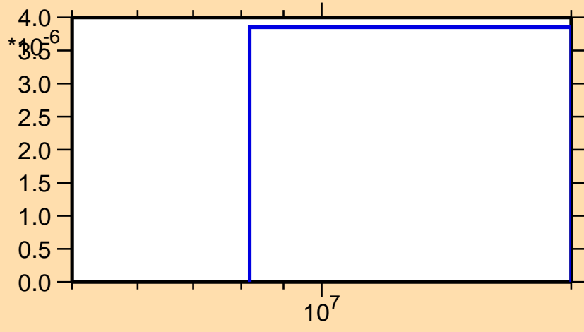
\sigma vs. E for ^{181}\text{Ir}(n,2n\alpha)
