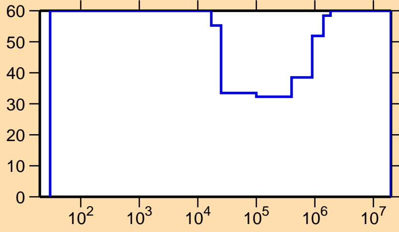
\Delta\sigma/\sigma vs. E for ^{181}\text{Ir}(n,\gamma)
