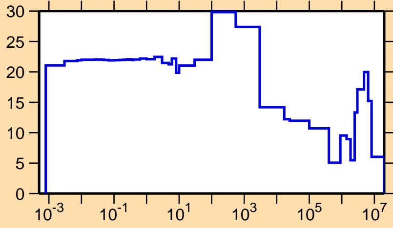
\Delta\sigma/\sigma vs. E for ^{181}\text{Ir}(n,\text{el.})
