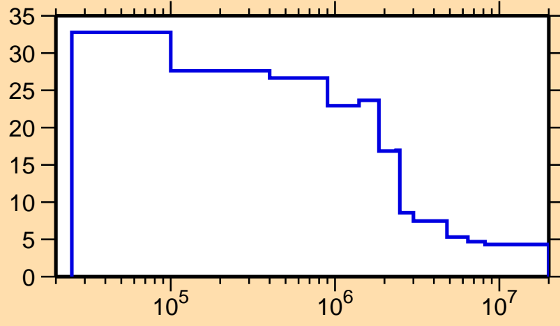
\Delta\sigma/\sigma vs. E for ^{181}\text{Ir}(n,\text{nonel.})
