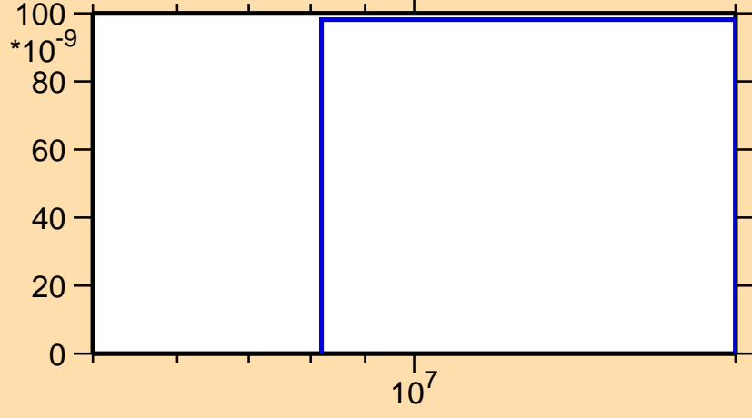
\sigma vs. E for ^{181}\text{Ir}(n,\text{nd})
