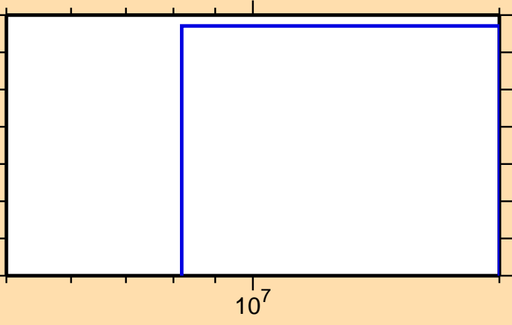
\sigma vs. E for ^{181}\text{Ir}(n,2np)
