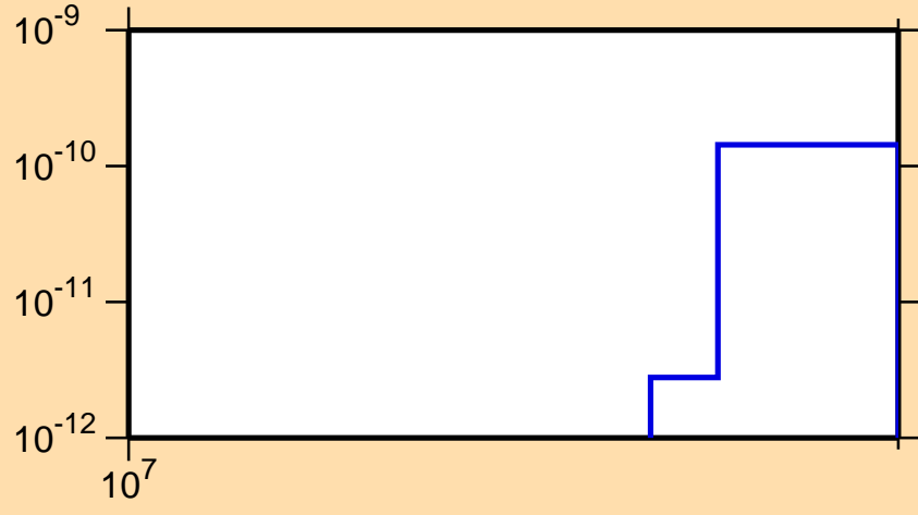
\sigma vs. E for ^{182}\text{Ir} (mt 34)
