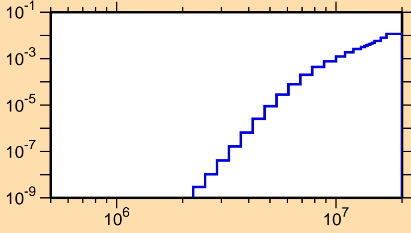
\sigma vs. E for ^{182}\text{Ir}(n,n\alpha)
