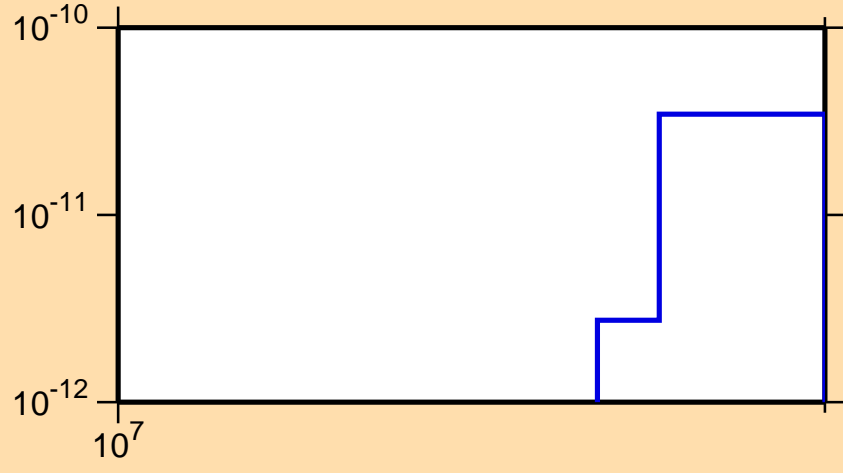
\sigma vs. E for ^{182}\text{Ir}(n,3n\alpha)
