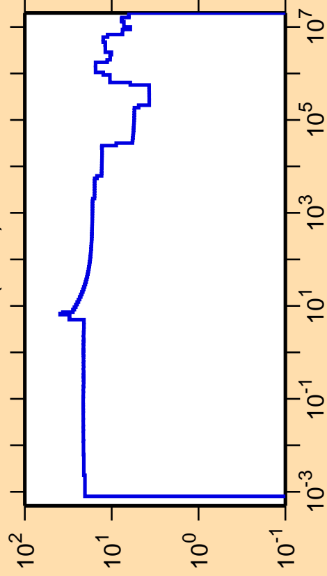
\Delta\sigma/\sigma vs. E for ^{182}\text{Ir}(n,\text{el.})
