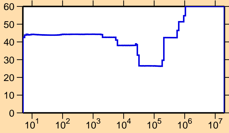
\Delta\sigma/\sigma vs. E for ^{182}\text{Ir}(n,\gamma)
