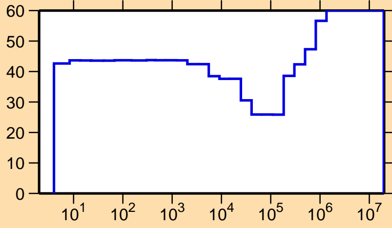
\Delta\sigma/\sigma vs. E for ^{182}\text{Ir}(n,\gamma)
