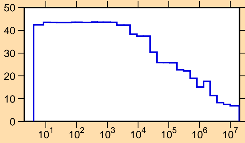
\Delta\sigma/\sigma vs. E for ^{182}\text{Ir}(n,\text{nonel.})
