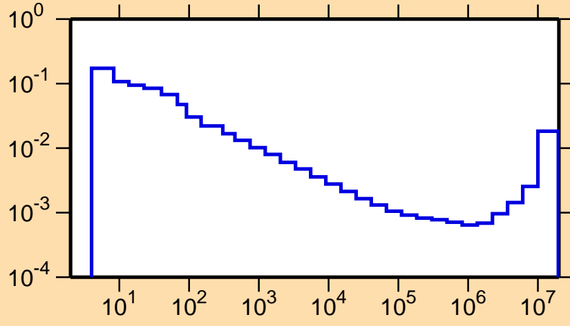
\sigma vs. E for ^{182}\text{Ir}(n,\alpha)
