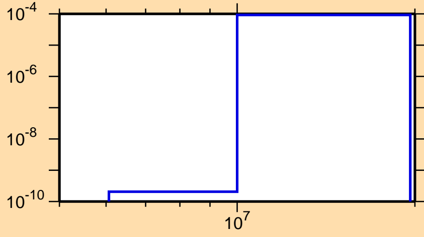
\sigma vs. E for ^{182}\text{Ir}(n,2n\alpha)
