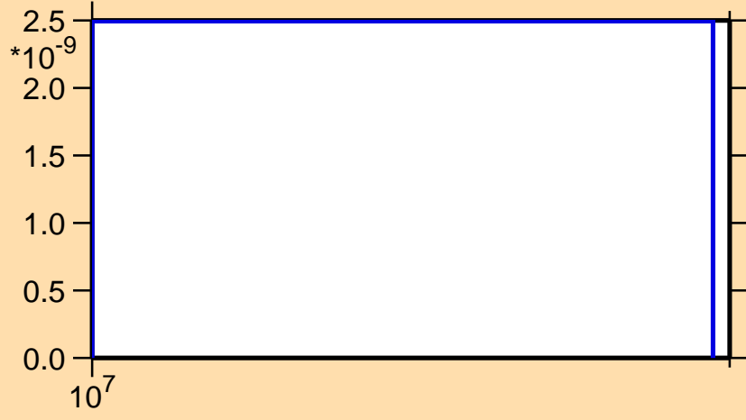
\sigma vs. E for ^{182}\text{Ir}(n,nt)
