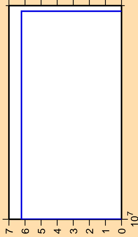
\Delta\sigma/\sigma vs. E for ^{182}\text{Ir} (mt 34)
