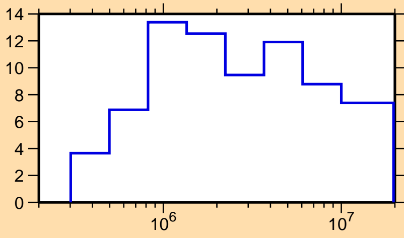
\Delta\sigma/\sigma vs. E for ^{182}\text{Ir}(n, el.)
