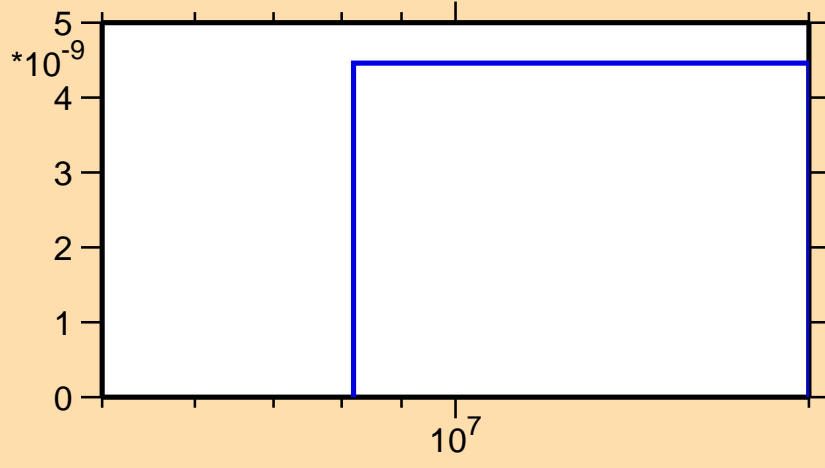
\sigma vs. E for ^{182}\text{Ir}(\text{mt117})
