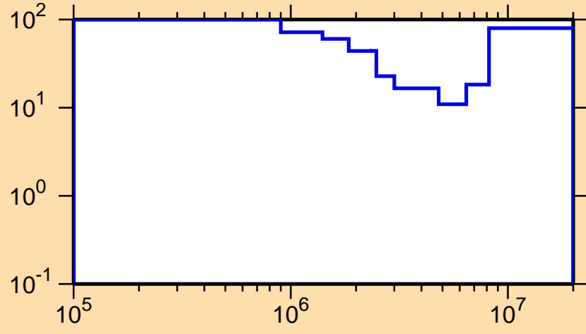
\Delta\sigma/\sigma vs. E for ^{182}\text{Ir}(n,n\text{cont.})
