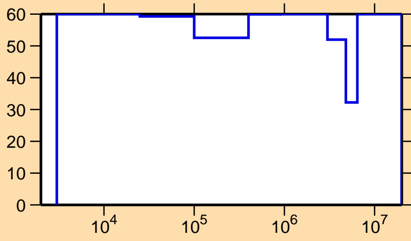
\Delta\sigma/\sigma vs. E for ^{182}\text{Ir}(n,n_1)
