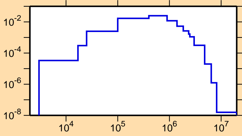
\sigma vs. E for ^{182}\text{Ir}(n,n_1)
