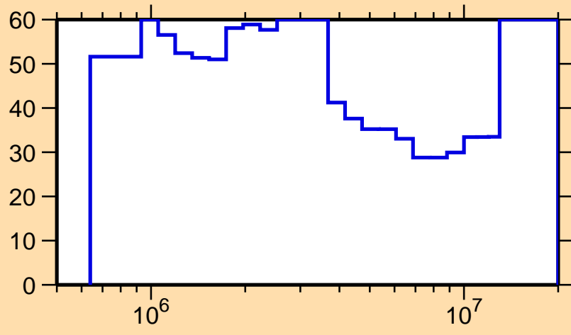
\Delta\sigma/\sigma vs. E for ^{183}\text{Ir}(n,n\text{cont.})
