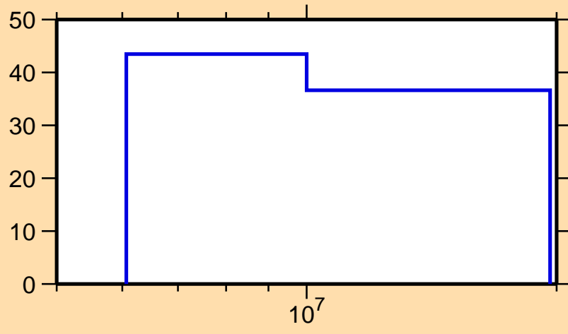
\Delta\sigma/\sigma vs. E for ^{183}\text{Ir}(n,2n)
