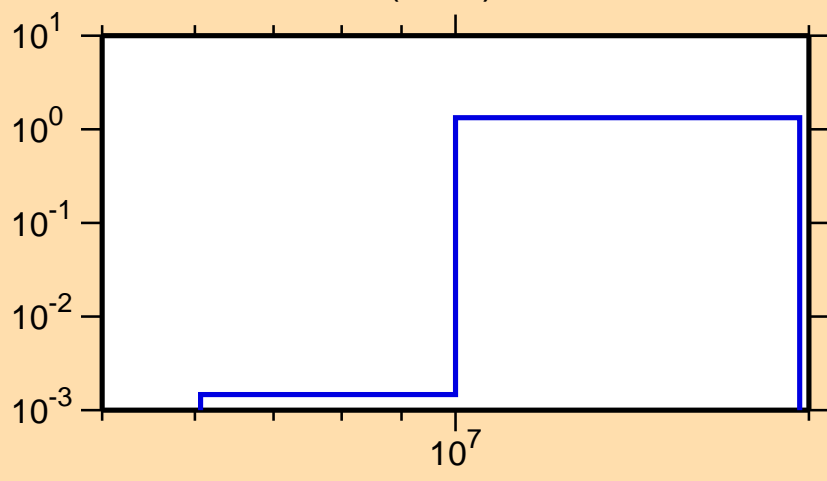
\sigma vs. E for ^{183}\text{Ir}(n,2n)
