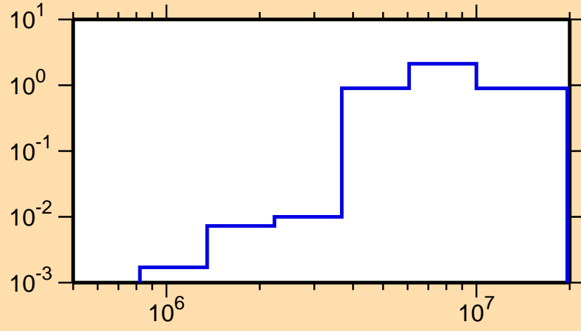
\sigma vs. E for ^{183}\text{Ir}(n,n\text{cont.})
