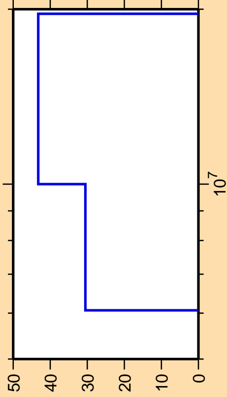
\Delta\sigma/\sigma vs. E for ^{183}\text{Ir}(n,n_1)
