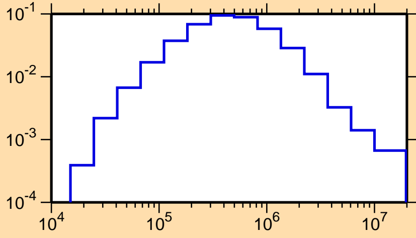
\sigma vs. E for ^{183}\text{Ir}(n,n_1)
