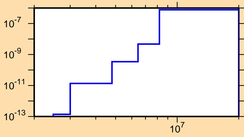
\sigma vs. E for ^{183}\text{Ir}(n,p\alpha)
