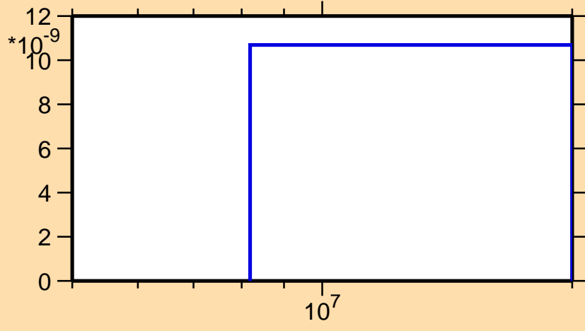
\sigma vs. E for ^{183}\text{Ir}(\text{mt } 45)
