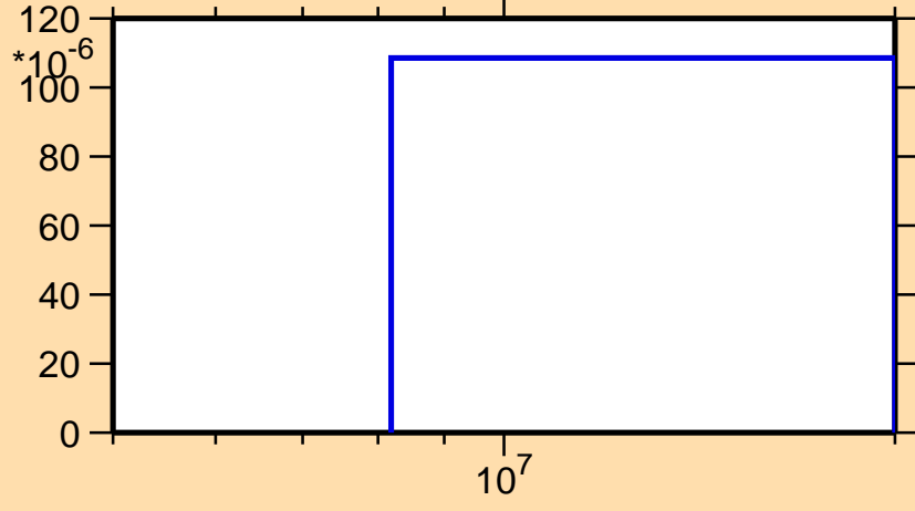
\sigma vs. E for ^{183}\text{Ir}(n,3n)
