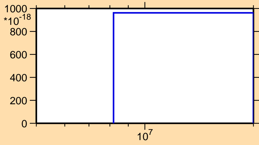
\sigma vs. E for ^{183}\text{Ir}(n,\text{pt})
