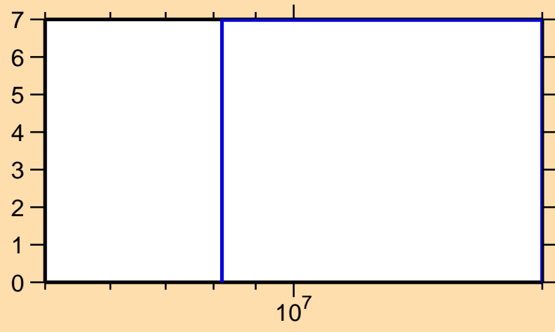
\Delta\sigma/\sigma vs. E for ^{183}\text{Ir}(n,\text{tot.})
