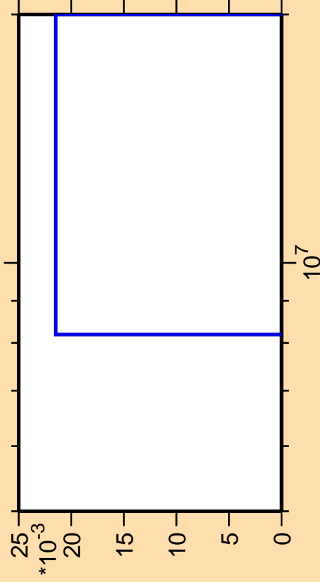
\Delta\sigma/\sigma vs. E for ^{183}\text{Ir}(\text{mt } 34)
