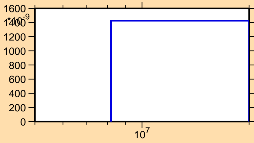
\sigma vs. E for ^{183}\text{Ir}(n,2np)
