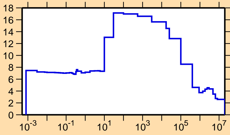
\sigma vs. E for ^{183}\text{Ir}(n,\text{el.})
