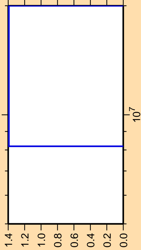
\Delta\sigma/\sigma vs. E for ^{183}\text{Ir}(n,3n\alpha)
