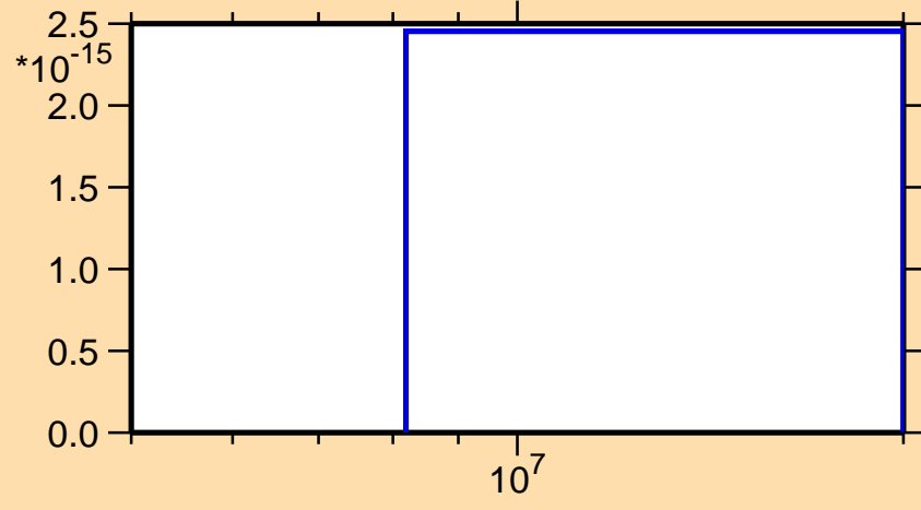
\sigma vs. E for ^{183}\text{Ir}(\text{mt } 34)
