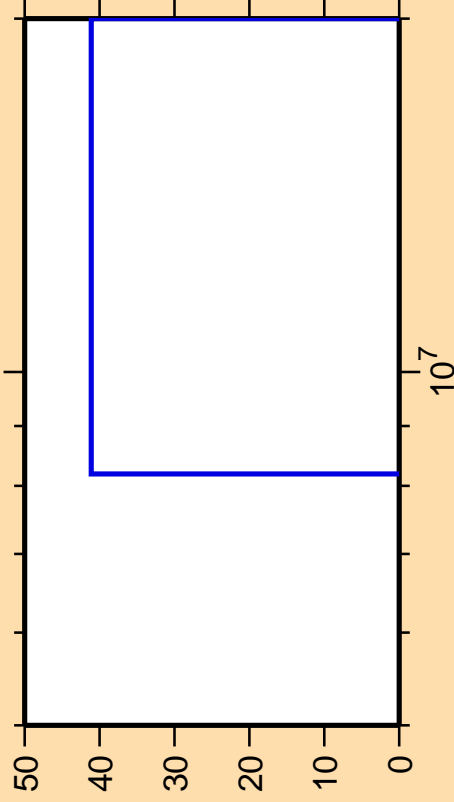
\Delta\sigma/\sigma vs. E for ^{183}\text{Ir}(n,n_1)
