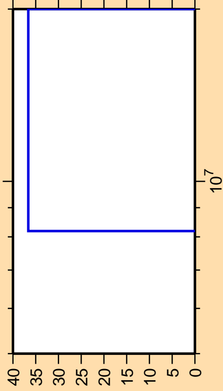
\Delta\sigma/\sigma vs. E for ^{183}\text{Ir}(n,2n)
