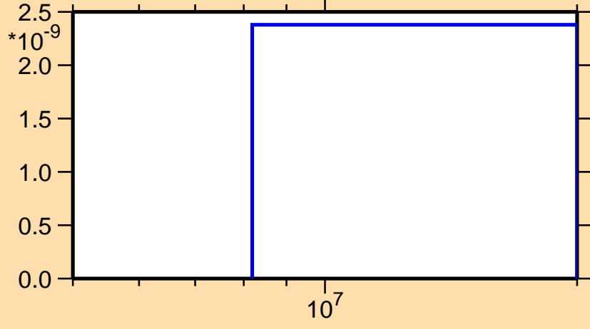
\sigma vs. E for ^{183}\text{Ir}(n,nt)
