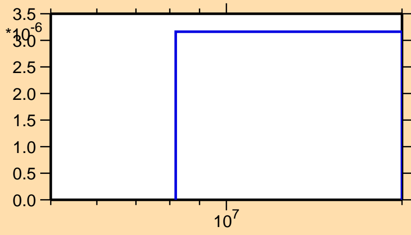
\sigma vs. E for ^{183}\text{Ir}(n,2n\alpha)
