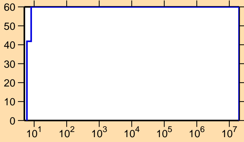
\Delta\sigma/\sigma vs. E for ^{184}\text{Ir}(n,p)
