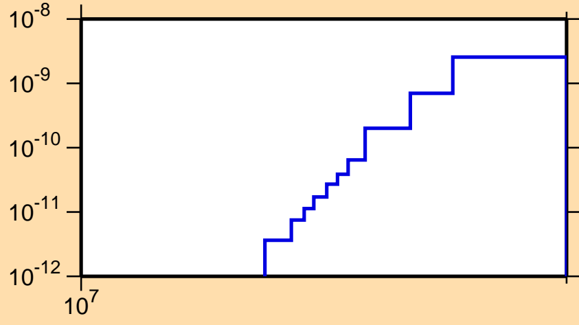
\sigma vs. E for ^{185}\text{Ir}(\text{mt117})
