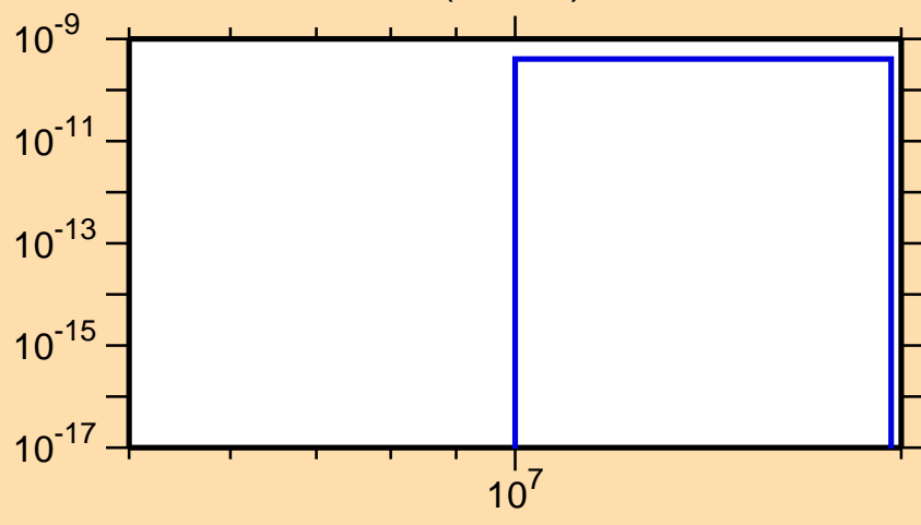
\sigma vs. E for ^{185}\text{Ir}(\text{mt } 45)
