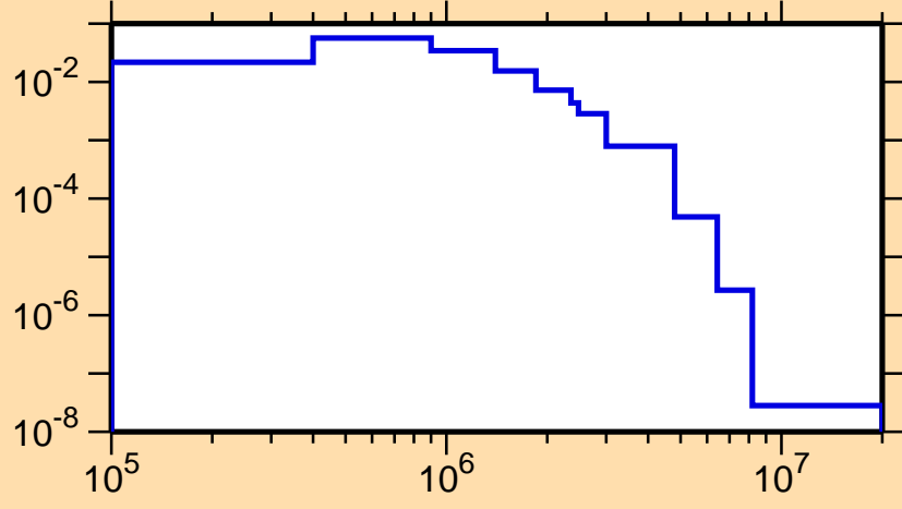
\sigma vs. E for ^{185}\text{Ir}(n,n_2)
