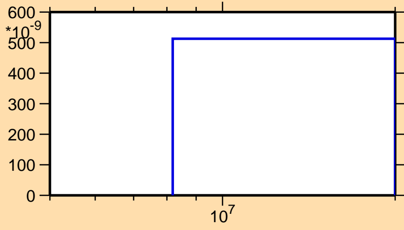
\sigma vs. E for ^{185}\text{Ir}(n,2n\alpha)
