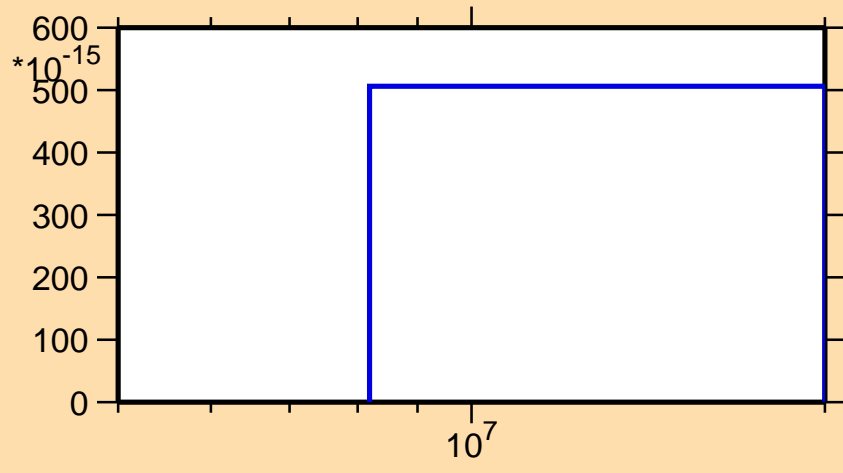
\sigma vs. E for ^{185}\text{Ir}(n,3n\alpha)
