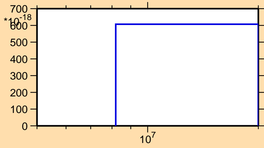
\sigma vs. E for ^{185}\text{Ir}(\text{mt } 34)
