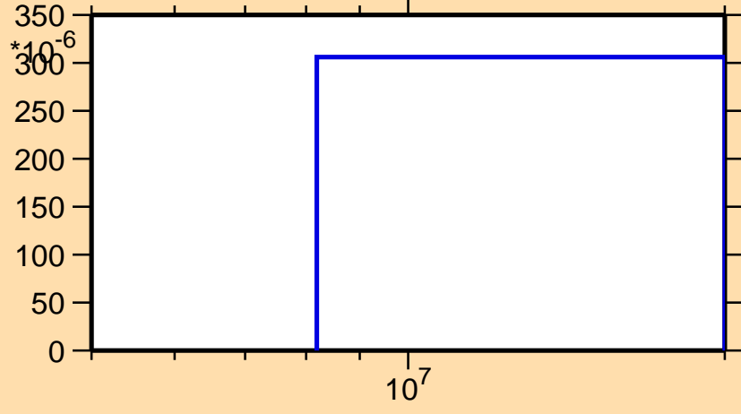
\sigma vs. E for ^{185}\text{Ir}(n,3n)
