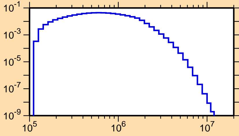
\sigma vs. E for ^{186}\text{Ir}(n,n_2)
