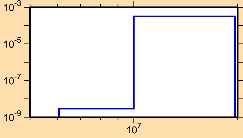
\sigma vs. E for ^{186}\text{Ir}(n,t)
