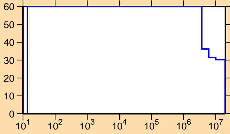
\Delta\sigma/\sigma vs. E for ^{186}\text{Ir}(n,p)
