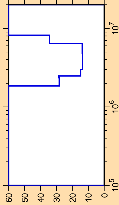
\Delta\sigma/\sigma vs. E for ^{186}\text{Ir}(n,\text{inel.})
