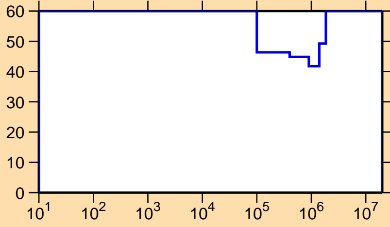
\Delta\sigma/\sigma vs. E for ^{186}\text{Ir}(n,\gamma)
