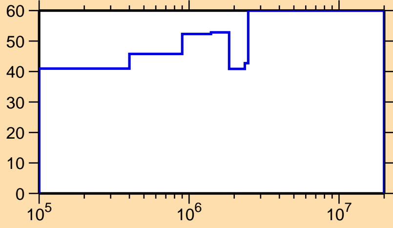
\Delta\sigma/\sigma vs. E for ^{186}\text{Ir}(n,n_1)
