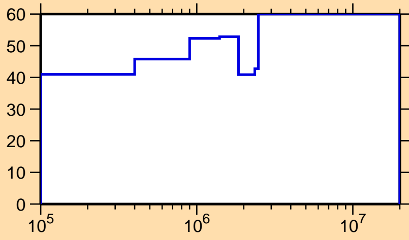
\Delta\sigma/\sigma vs. E for ^{186}\text{Ir}(n,n_1)
