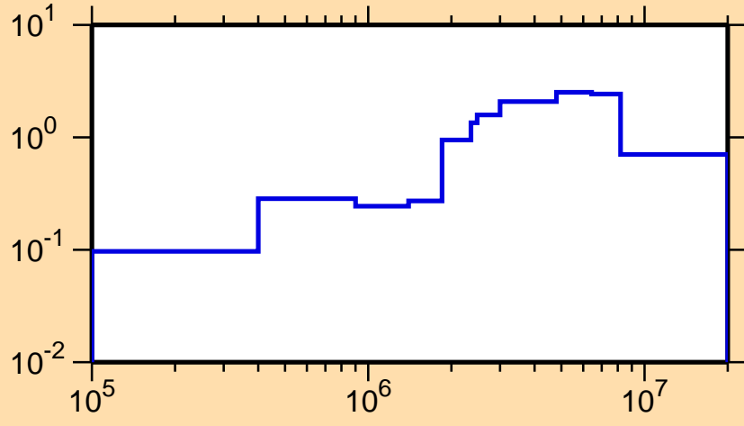
\sigma vs. E for ^{186}\text{Ir}(n,\text{inel.})
