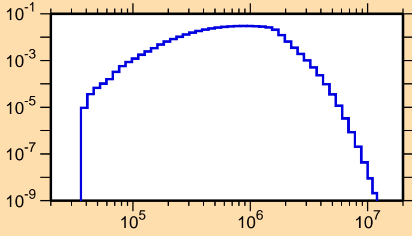
\sigma vs. E for ^{186}\text{Ir}(n,n_3)
