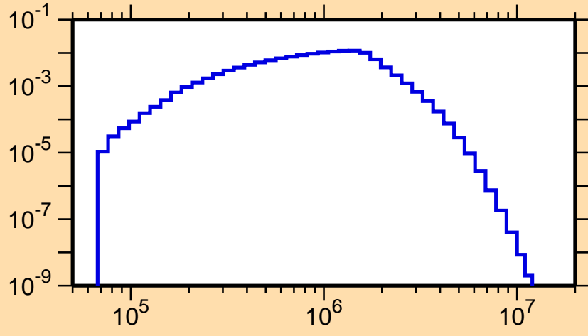
\sigma vs. E for ^{186}\text{Ir}(n,n_4)
