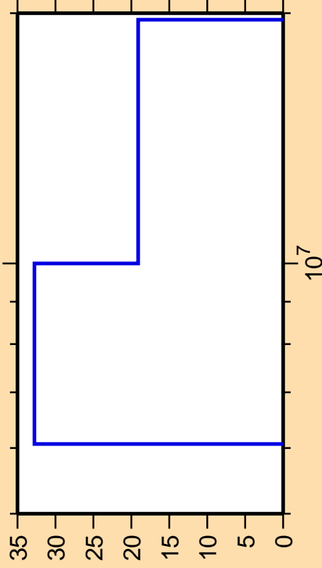
\Delta\sigma/\sigma vs. E for ^{186}\text{Ir}(n,2n)
