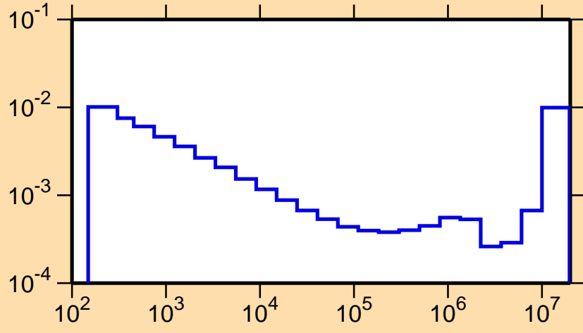
\sigma vs. E for ^{186}\text{Ir}(n,\alpha)
