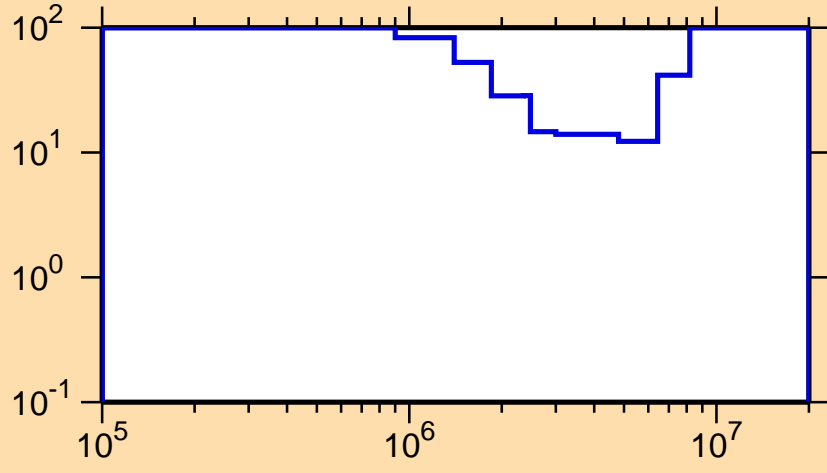
\Delta\sigma/\sigma vs. E for ^{186}\text{Ir}(n,n\text{cont.})
