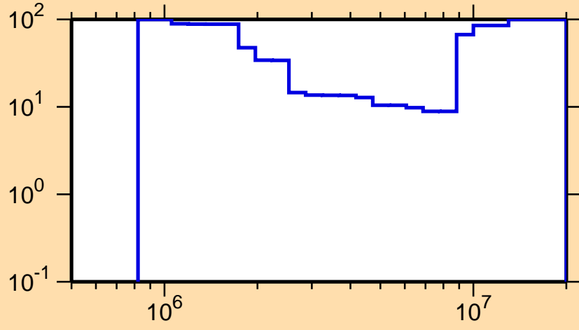
\Delta\sigma/\sigma vs. E for ^{187}\text{Ir}(n,n\text{cont.})
