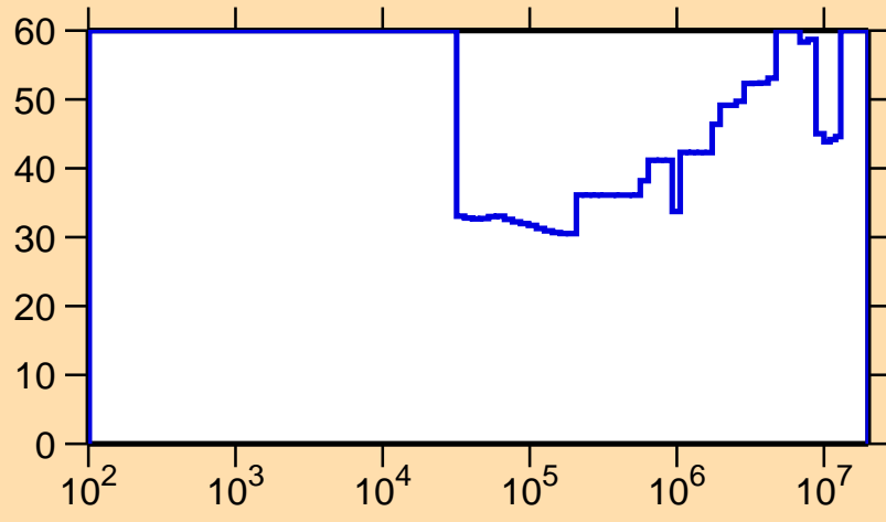
\Delta\sigma/\sigma vs. E for ^{187}\text{Ir}(n,\gamma)
