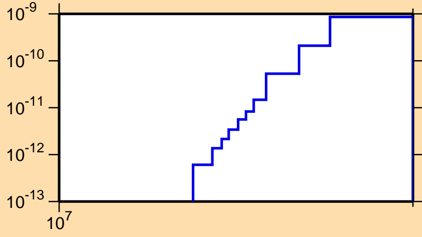
\sigma vs. E for ^{187}\text{Ir}(\text{mt117})
