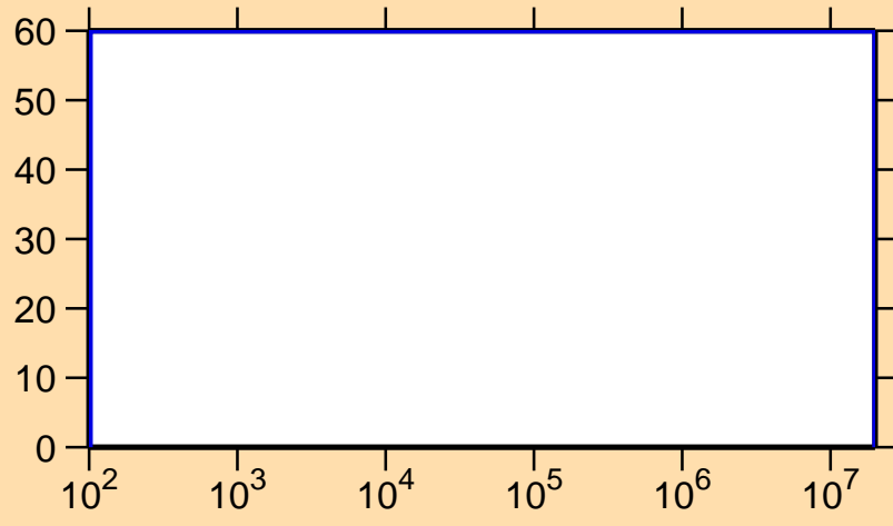
\Delta\sigma/\sigma vs. E for ^{187}\text{Ir}(n,p)
