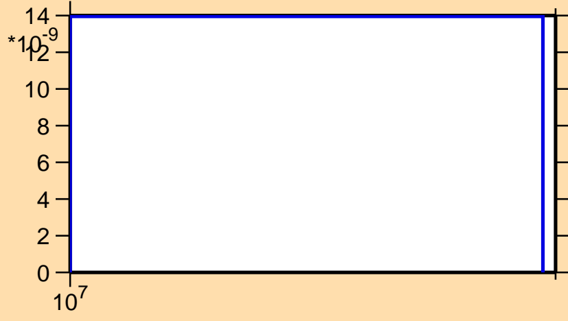
\sigma vs. E for ^{187}\text{Ir}(n,nt)
