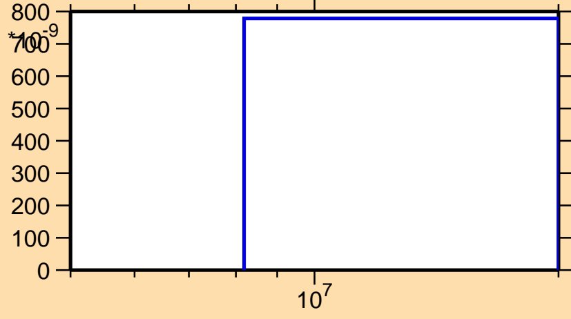
\sigma vs. E for ^{187}\text{Ir}(n,2n\alpha)
