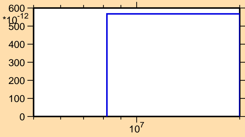
\sigma vs. E for ^{187}\text{Ir}(n,\text{He}3)
