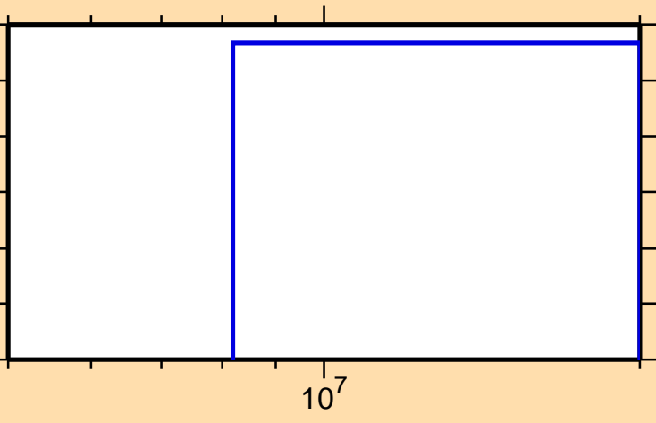
\sigma vs. E for ^{187}\text{Ir}(n,\text{He}3)
