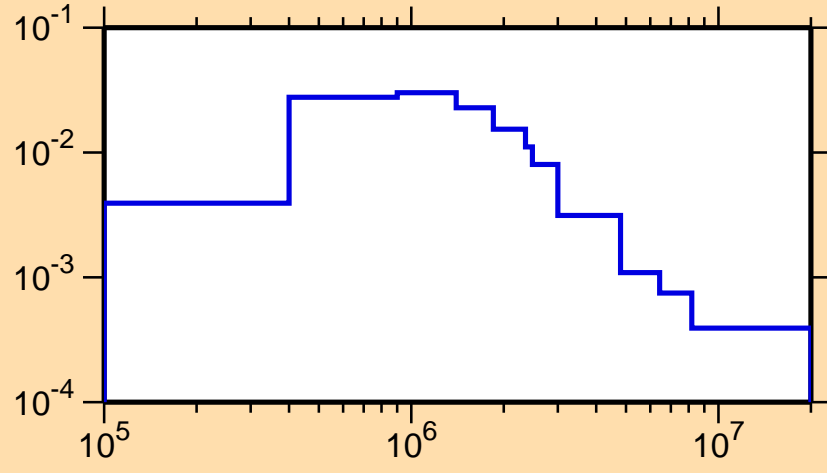
\sigma vs. E for ^{187}\text{Ir}(n,n_3)
