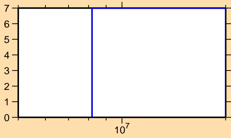
\Delta\sigma/\sigma vs. E for ^{187}\text{Ir}(n,\text{nonel.})
