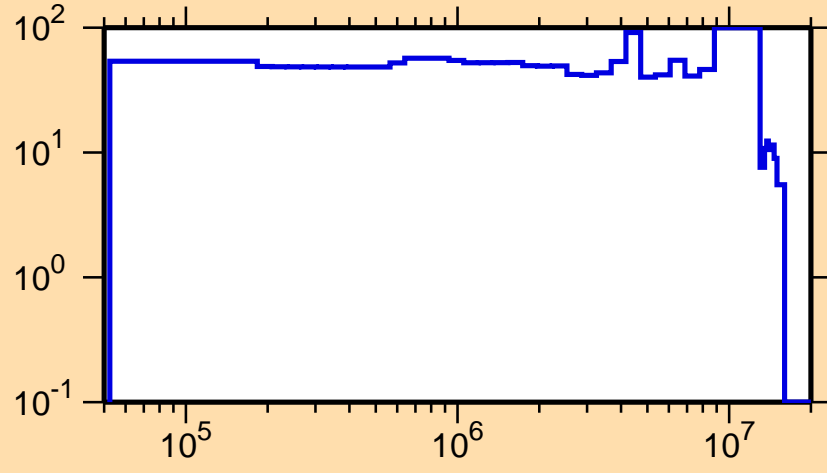
\Delta\sigma/\sigma vs. E for ^{188}\text{Ir}(n,n_1)
