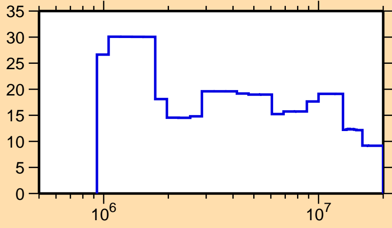
\Delta\sigma/\sigma vs. E for ^{188}\text{Ir}(n,el.)
