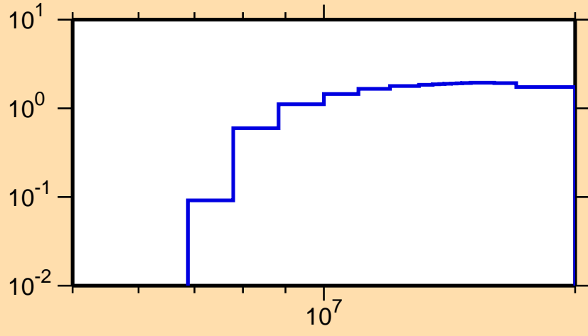
\sigma vs. E for ^{188}\text{Ir}(n,2n)
