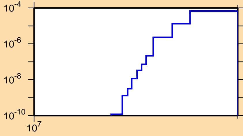
\sigma vs. E for ^{188}\text{Ir}(n,2np)
