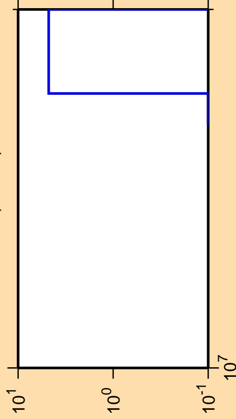
\Delta\sigma/\sigma vs. E for ^{188}\text{Ir}(\text{mt } 34)
