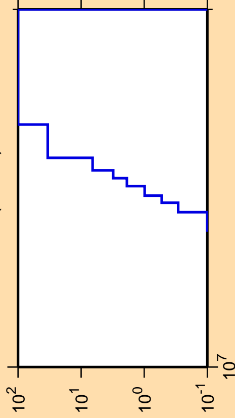
\Delta\sigma/\sigma vs. E for ^{188}\text{Ir}(\text{mt } 45)
