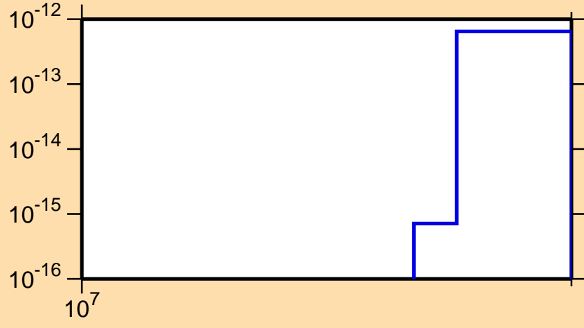
\sigma vs. E for ^{188}\text{Ir}(\text{mt } 34)
