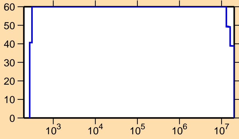
\Delta\sigma/\sigma vs. E for ^{188}\text{Ir}(n,p)
