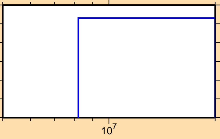
\sigma vs. E for ^{188}\text{Ir}(\text{mt } 34)
