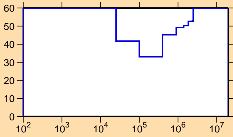
\Delta\sigma/\sigma vs. E for ^{188}\text{Ir}(n,\gamma)
