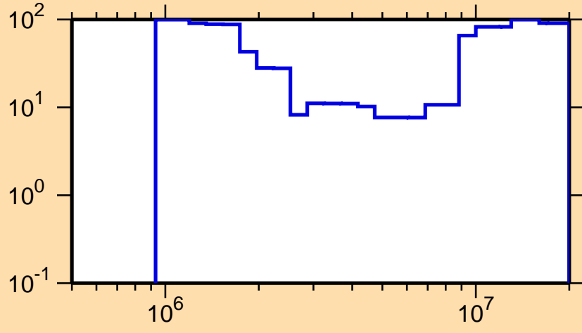
\Delta\sigma/\sigma vs. E for ^{189}\text{Ir}(n,n\text{cont.})
