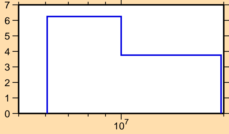
\Delta\sigma/\sigma vs. E for ^{189}\text{Ir}(n,\text{tot.})
