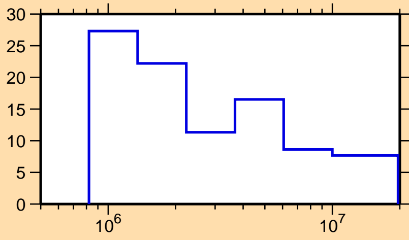
\Delta\sigma/\sigma vs. E for ^{189}\text{Ir}(n, el.)
