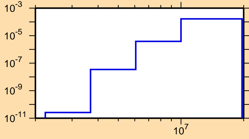
\sigma vs. E for ^{189}\text{Ir}(n,n\alpha)
