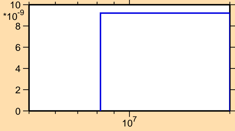
\sigma vs. E for ^{189}\text{Ir}(n,nt)
