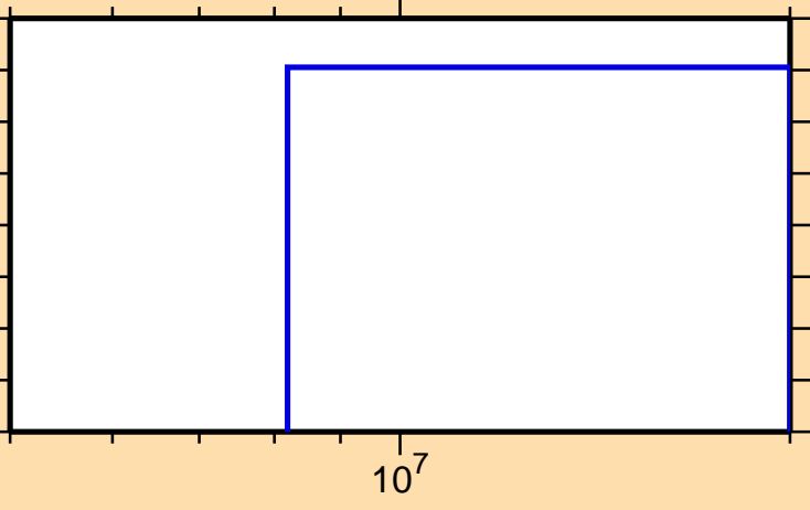
\sigma vs. E for ^{189}\text{Ir}(n,3n)
