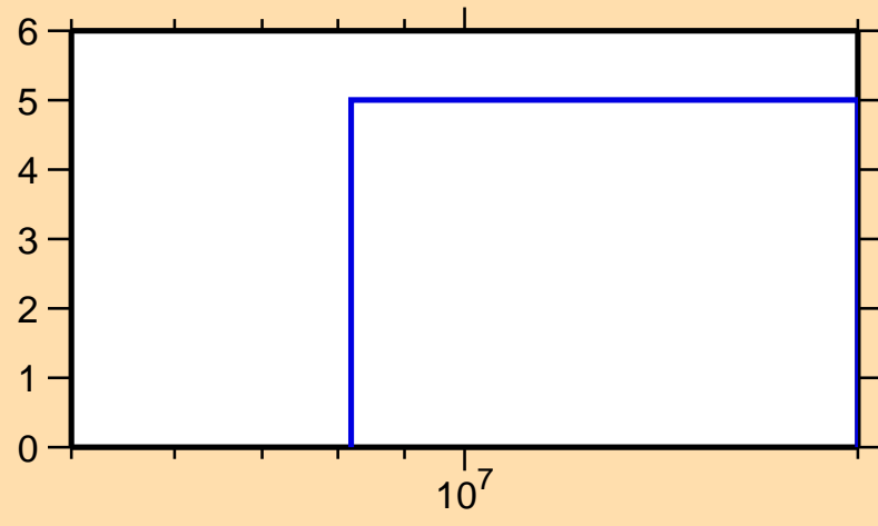
\Delta\sigma/\sigma vs. E for ^{189}\text{Ir}(n,\text{nonel.})
