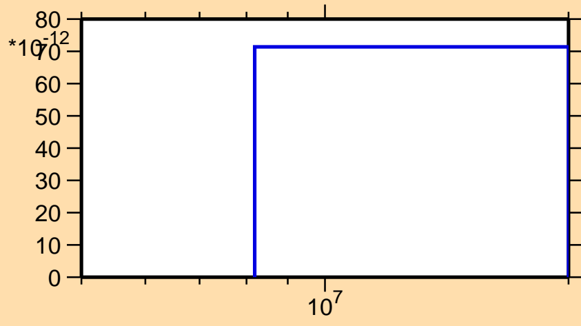
\sigma vs. E for ^{189}\text{Ir}(n,p\alpha)
