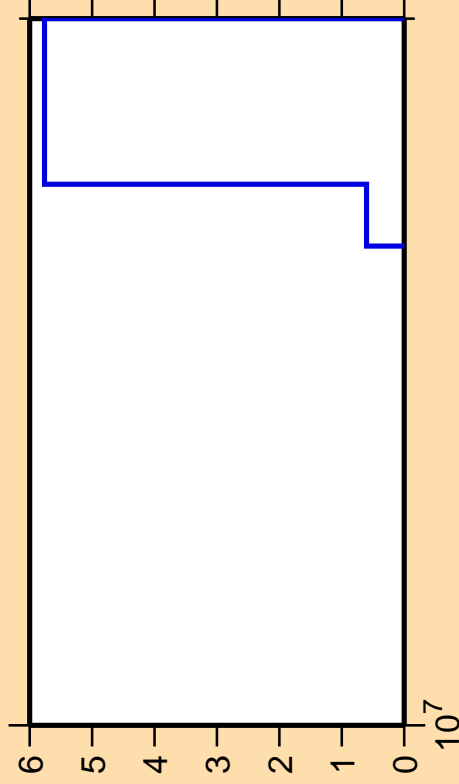
\Delta\sigma/\sigma vs. E for ^{190}\text{Ir} (mt 45)
