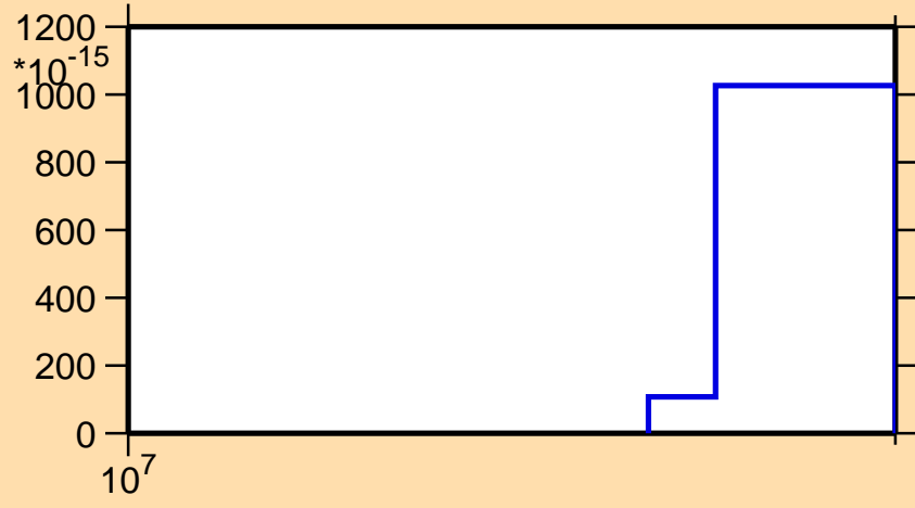
\sigma vs. E for ^{190}\text{Ir} (mt 45)
