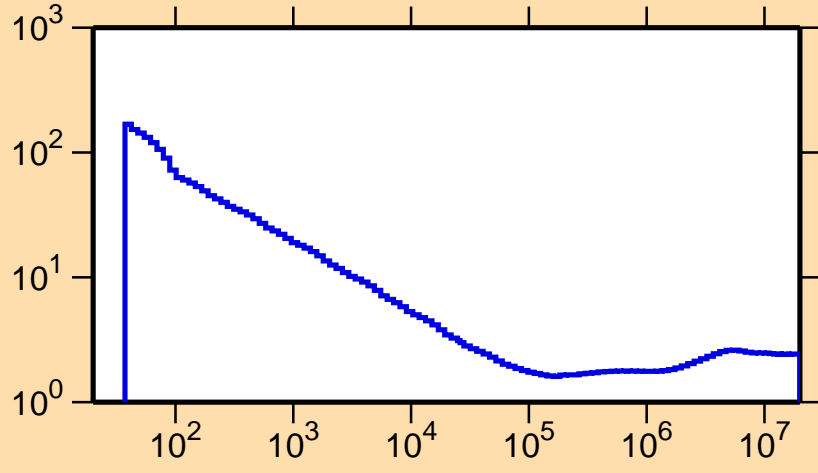
\sigma vs. E for ^{190}\text{Ir}(n,\text{nonel.})
