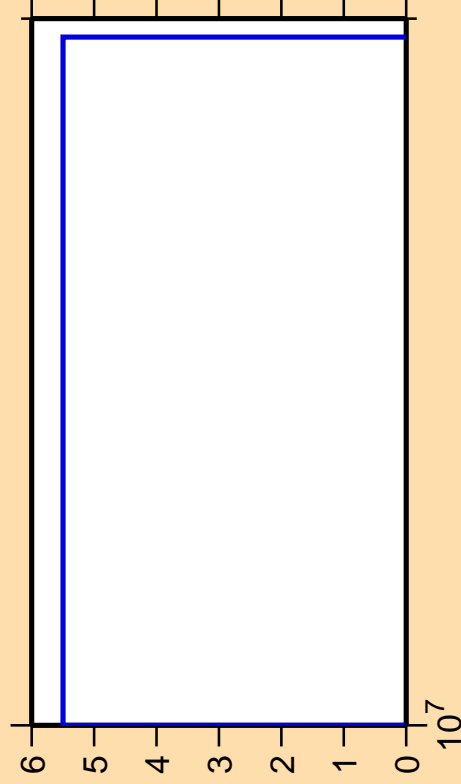
\Delta\sigma/\sigma vs. E for ^{190}\text{Ir}(n,3n\alpha)
