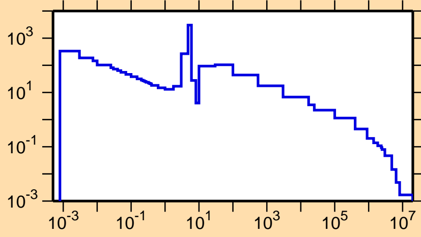
\sigma vs. E for ^{190}\text{Ir}(n,\gamma)
