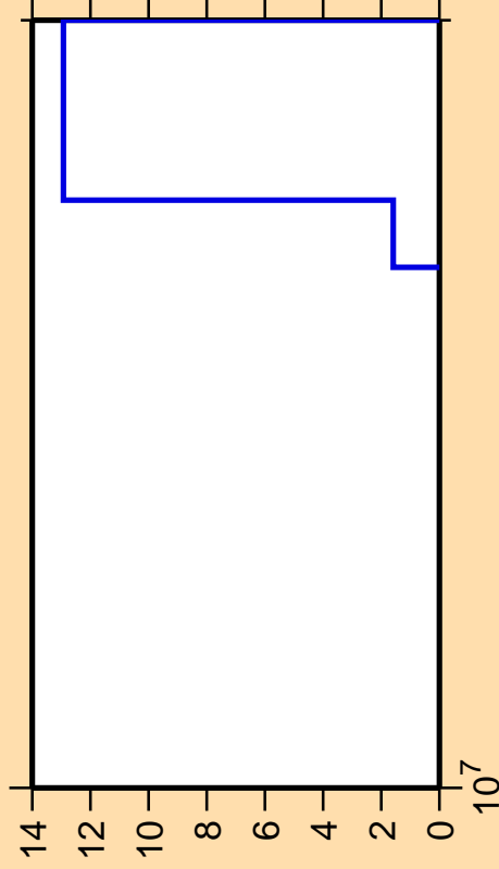
\Delta\sigma/\sigma vs. E for ^{190}\text{Ir} (mt 45)
