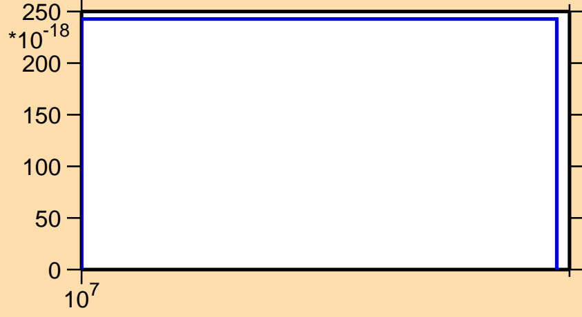
\sigma vs. E for ^{190}\text{Ir} (mt 34)
