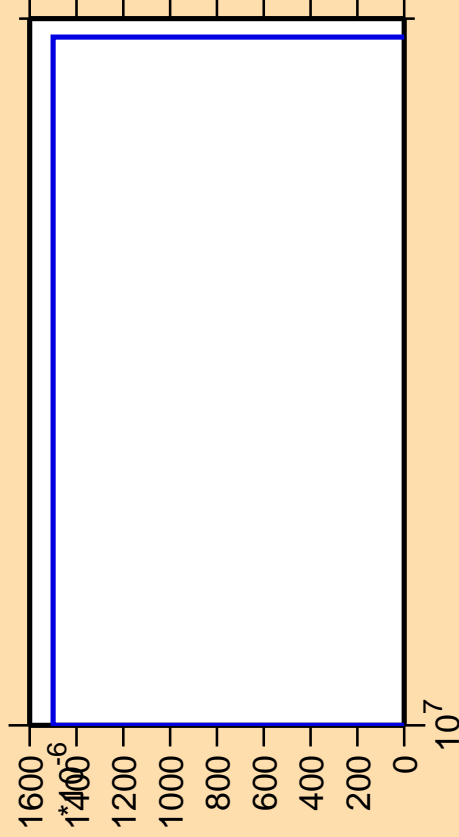
\Delta\sigma/\sigma vs. E for ^{190}\text{Ir} (mt 34)
