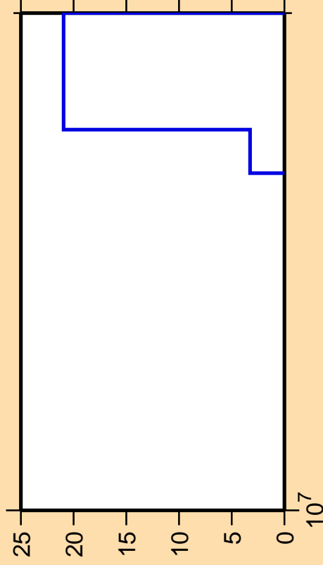
\Delta\sigma/\sigma vs. E for ^{190}\text{Ir}(\text{mt117})
