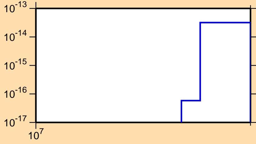
\sigma vs. E for ^{190}\text{Ir} (mt 34)
