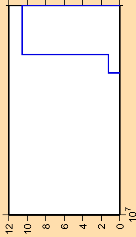
\Delta\sigma/\sigma vs. E for ^{190}\text{Ir}(\text{mt } 45)
