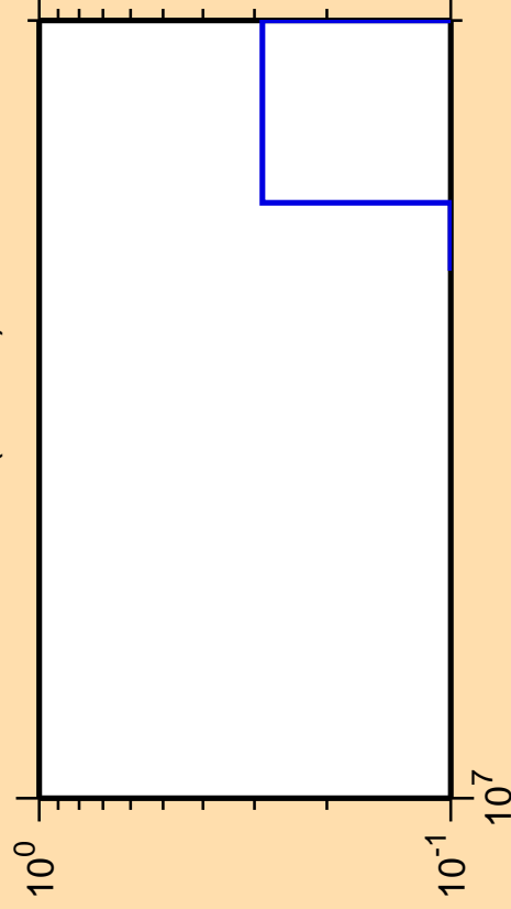
\Delta\sigma/\sigma vs. E for ^{190}\text{Ir} (mt 34)
