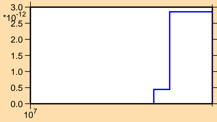
\sigma vs. E for ^{190}\text{Ir}(\text{mt117})
