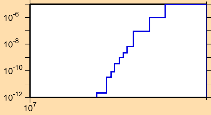
\sigma vs. E for ^{190}\text{Ir}(n,2np)
