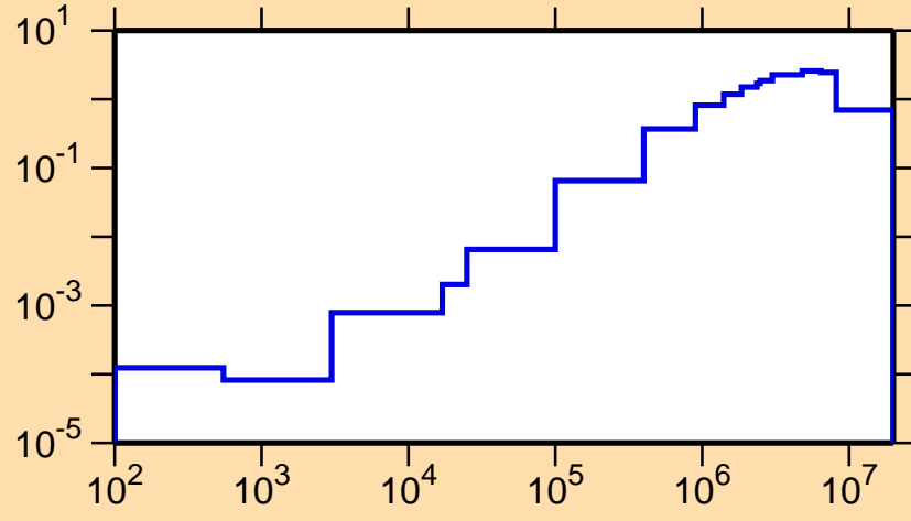
\sigma vs. E for ^{190}\text{Ir}(n,n\text{cont.})
