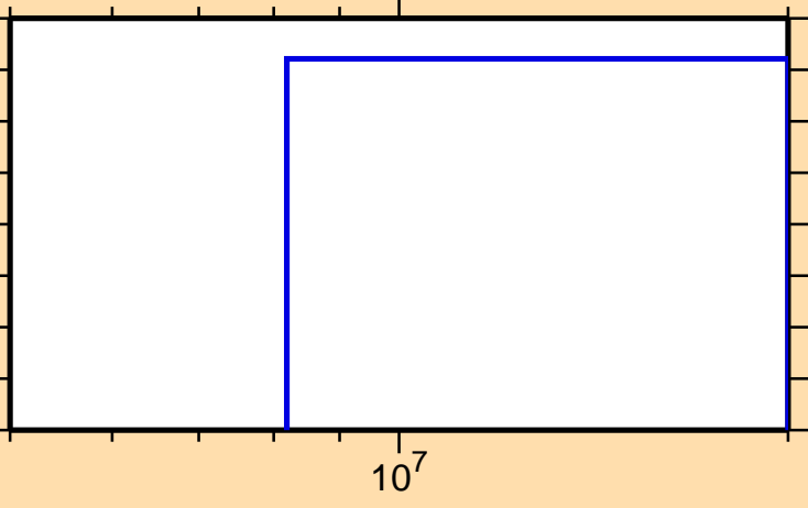
\sigma vs. E for ^{190}\text{Ir}(n,nt)
