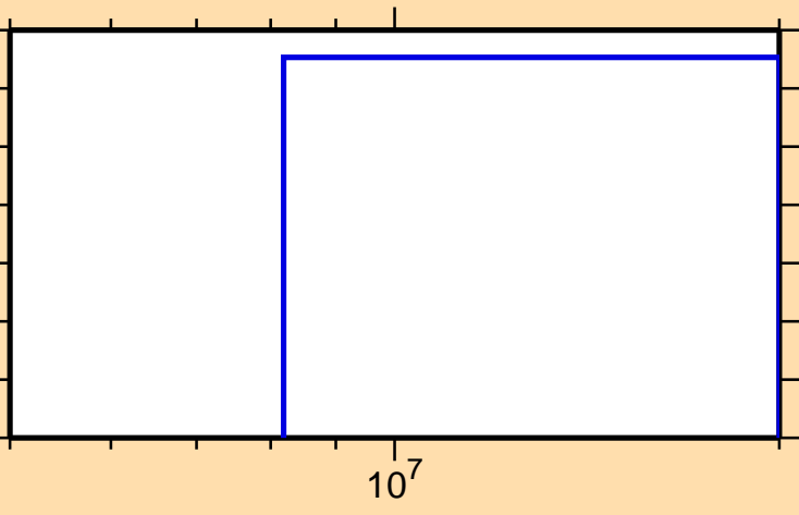
\sigma vs. E for ^{190}\text{Ir}(n,2np)
