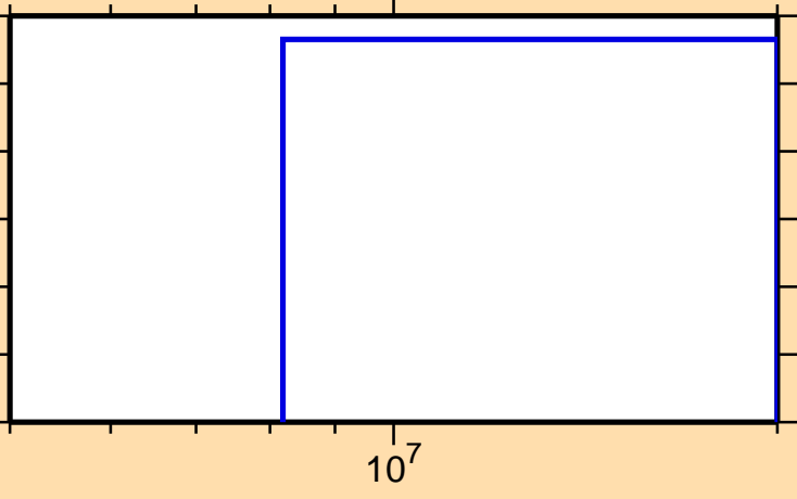
\sigma vs. E for ^{190}\text{Ir}(n,\text{nd})
