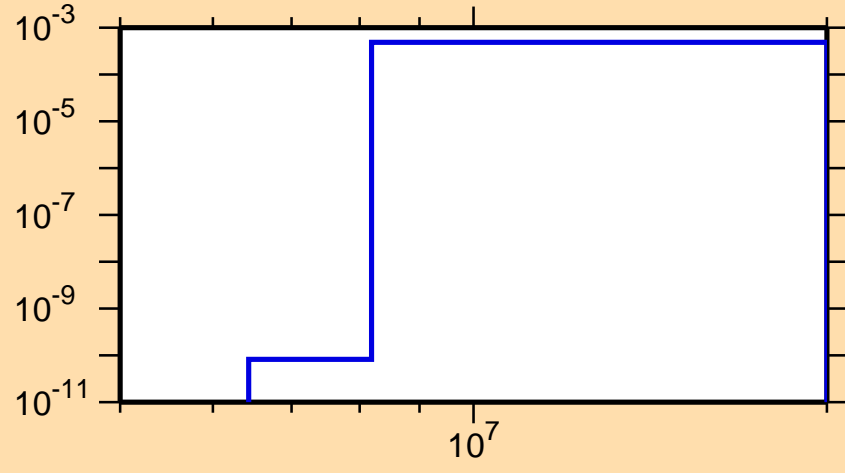
\sigma vs. E for ^{190}\text{Ir}(n,np)
