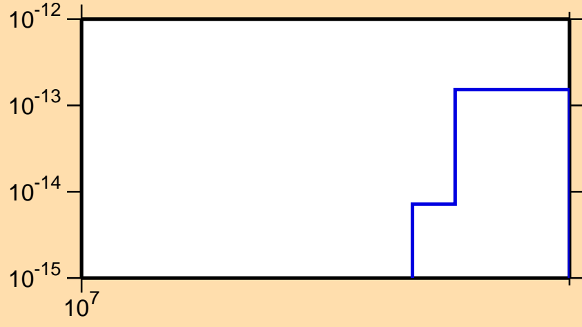
\sigma vs. E for ^{191}\text{Ir} (mt 45)
