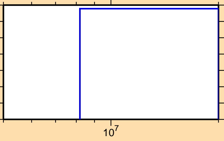
\sigma vs. E for ^{191}\text{Ir}(n,\text{nd})
