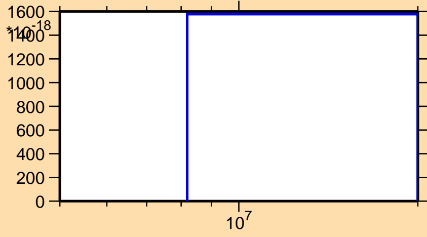
\sigma vs. E for ^{191}\text{Ir}(\text{mt } 45)
