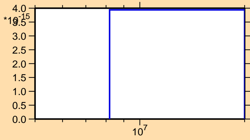
\sigma vs. E for ^{191}\text{Ir}(\text{mt117})
