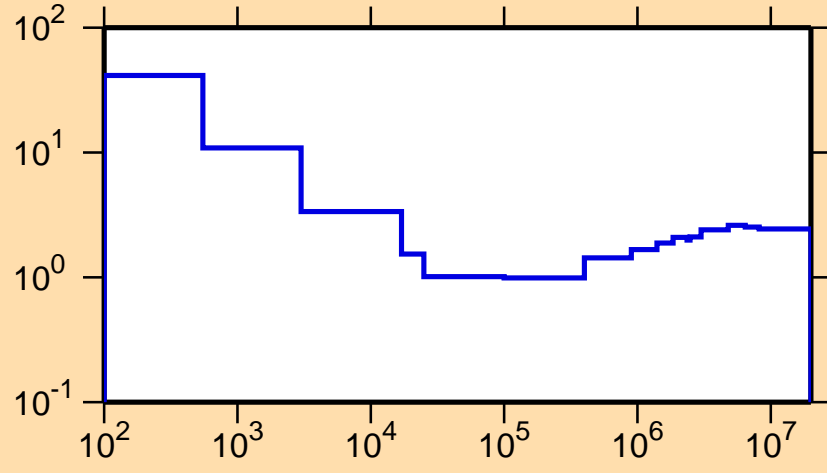
\sigma vs. E for ^{191}\text{Ir}(n,\text{nonel.})
