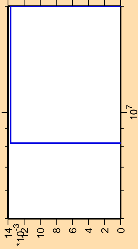
\Delta\sigma/\sigma vs. E for ^{191}\text{Ir}(\text{mt } 45)
