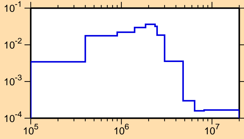
\sigma vs. E for ^{191}\text{Ir}(n,n_3)
