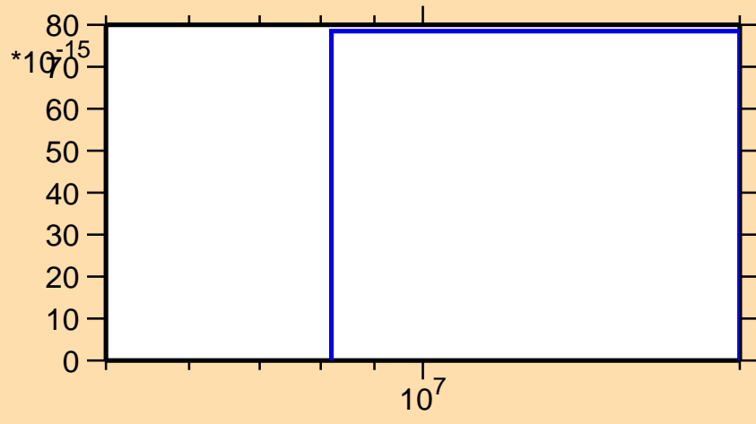
\sigma vs. E for ^{191}\text{Ir}(\text{mt } 45)
