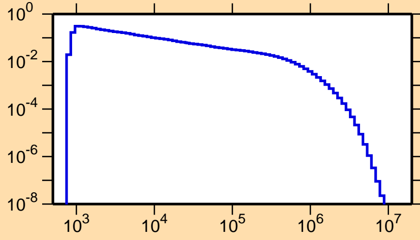
\sigma vs. E for ^{191}\text{Ir}(n,n_2)
