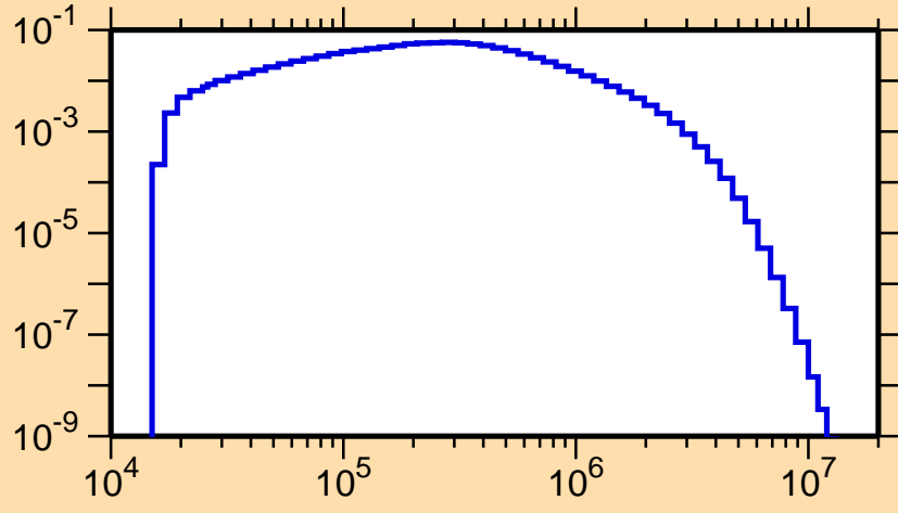
\sigma vs. E for ^{192}\text{Ir}(n,n_2)
