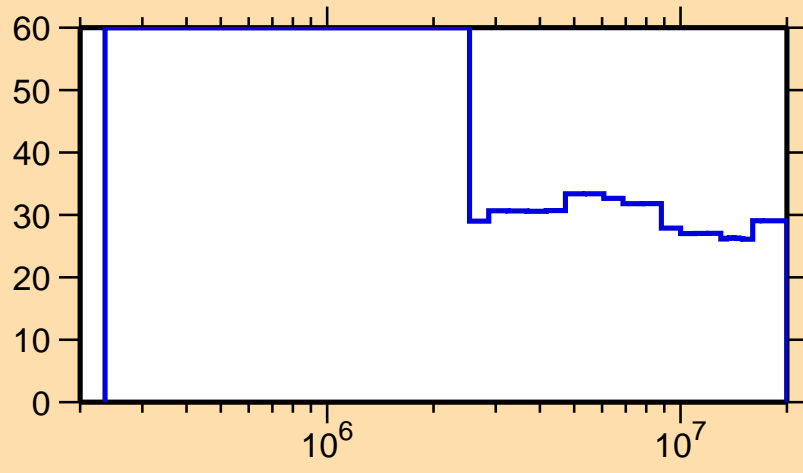
\Delta\sigma/\sigma vs. E for ^{192}\text{Ir}(n,n_1)
