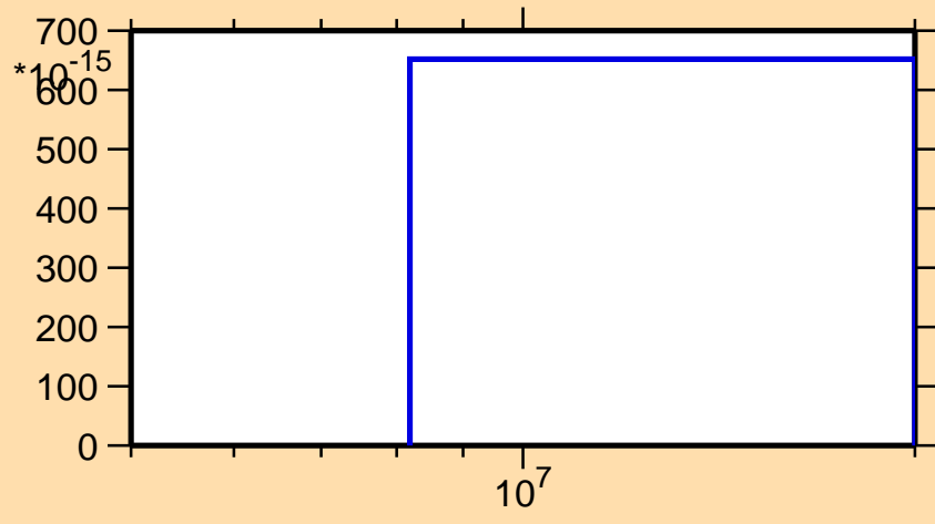
\sigma vs. E for ^{192}\text{Ir}(n,p\alpha)
