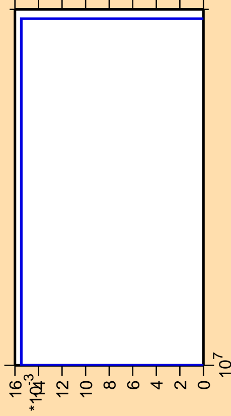
\Delta\sigma/\sigma vs. E for ^{193}\text{Ir}(n,3n\alpha)
