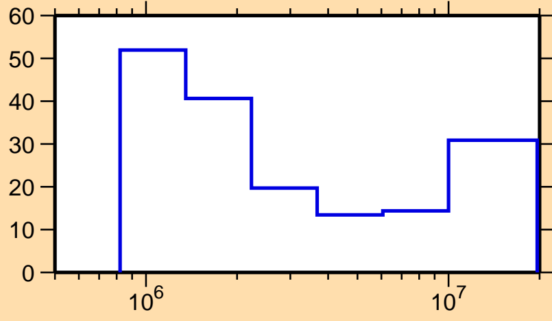
\Delta\sigma/\sigma vs. E for ^{193}\text{Ir}(n,n\text{cont.})
