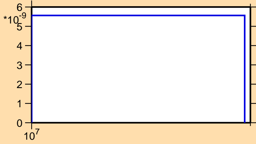
\sigma vs. E for ^{193}\text{Ir}(n,2n\alpha)
