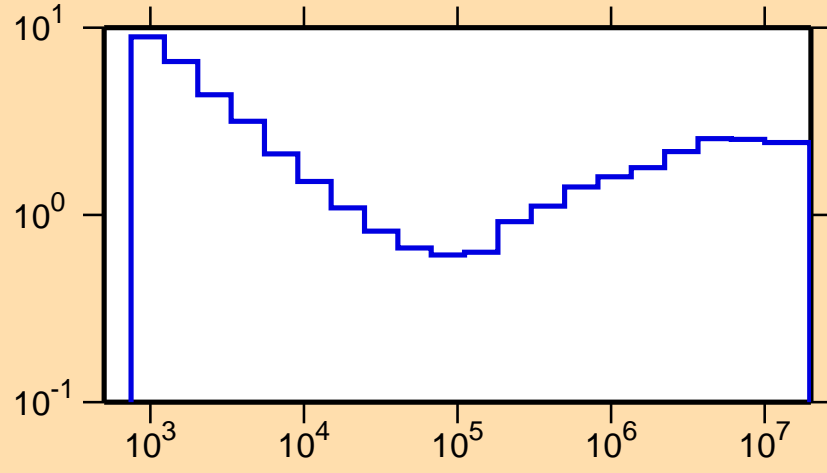
\sigma vs. E for ^{193}\text{Ir}(n,\text{nonel.})
