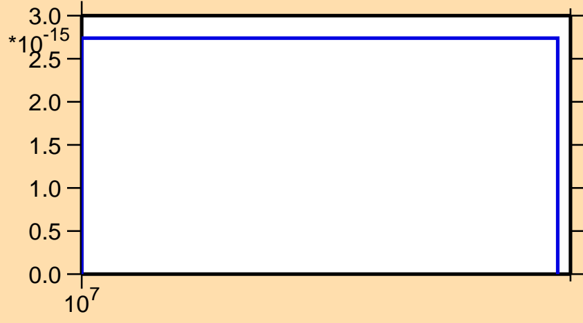
\sigma vs. E for ^{193}\text{Ir}(n,3n\alpha)
