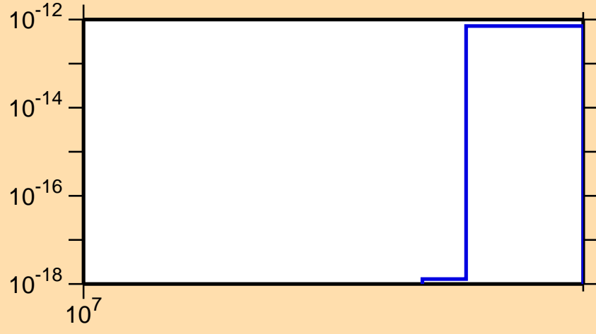
\sigma vs. E for ^{193}\text{Ir}(n,3n\alpha)
