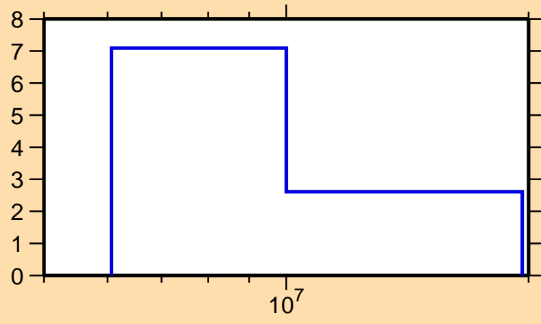
\Delta\sigma/\sigma vs. E for ^{194}\text{Ir}(n,\text{tot.})
