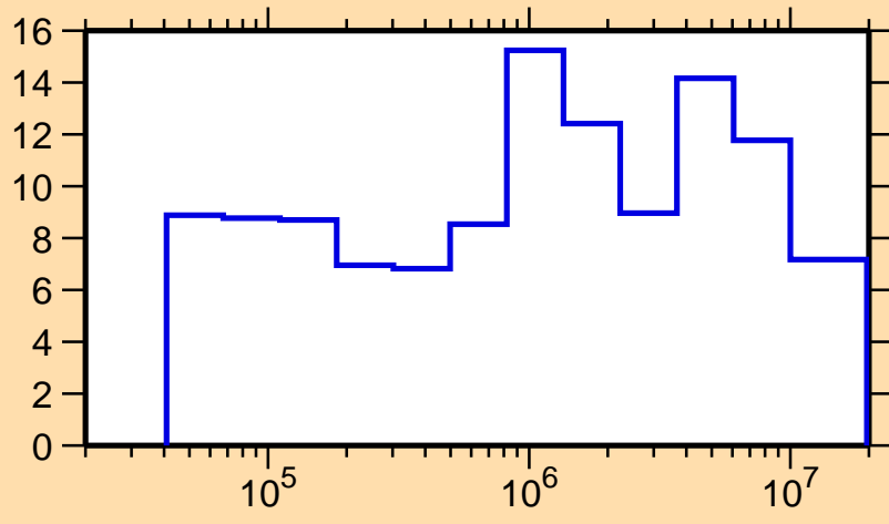
\Delta\sigma/\sigma vs. E for ^{194}\text{Ir}(n,\text{el.})
