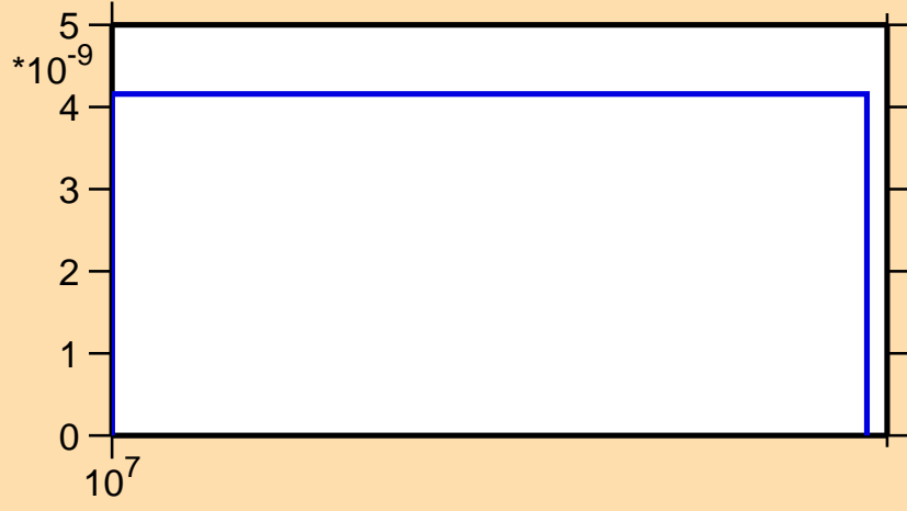
\sigma vs. E for ^{194}\text{Ir}(n,nt)
