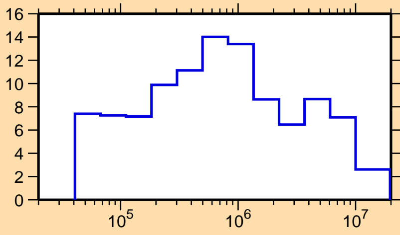
\Delta\sigma/\sigma vs. E for ^{194}\text{Ir}(n,\text{tot.})
