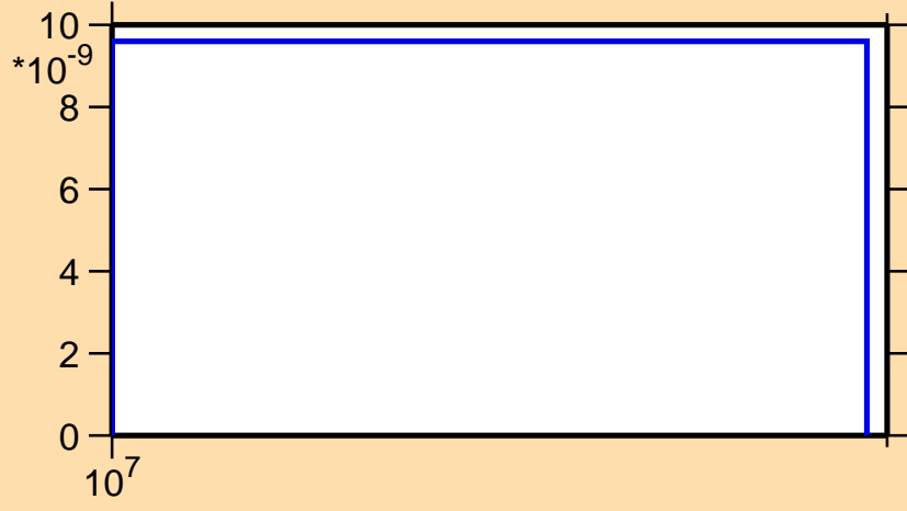
\sigma vs. E for ^{194}\text{Ir}(n,2np)
