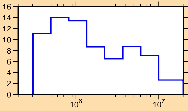
\Delta\sigma/\sigma vs. E for ^{194}\text{Ir}(n, tot.)
