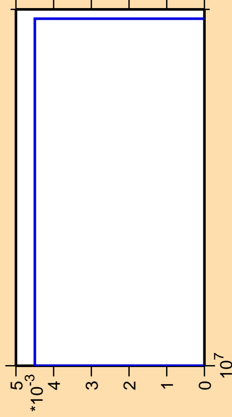
\Delta\sigma/\sigma vs. E for ^{194}\text{Ir}(n,3n\alpha)
