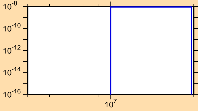
\sigma vs. E for ^{194}\text{Ir}(n,2n\alpha)
