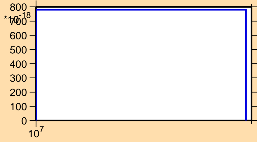
\sigma vs. E for ^{194}\text{Ir}(n,3n\alpha)
