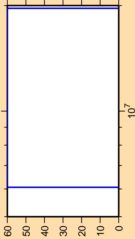
\Delta\sigma/\sigma vs. E for ^{194}\text{Ir}(n,d)
