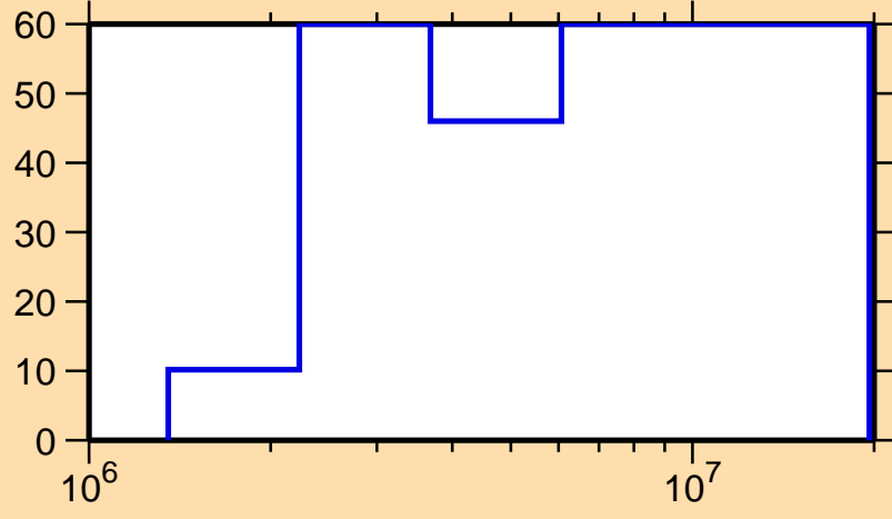
\Delta\sigma/\sigma vs. E for ^{194}\text{Ir}(n,p)
