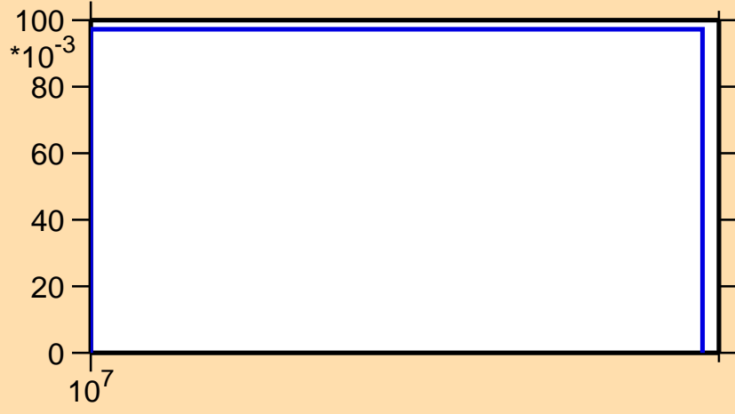
\sigma vs. E for ^{194}\text{Ir}(n,3n)
