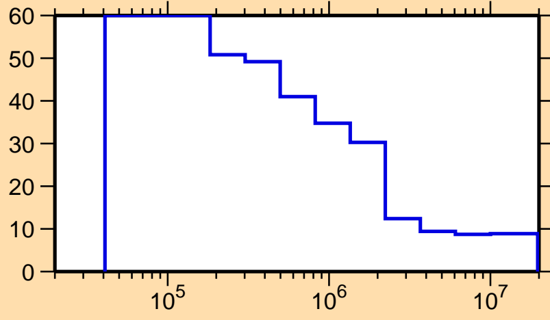
\Delta\sigma/\sigma vs. E for ^{194}\text{Ir}(n,\text{nonel.})
