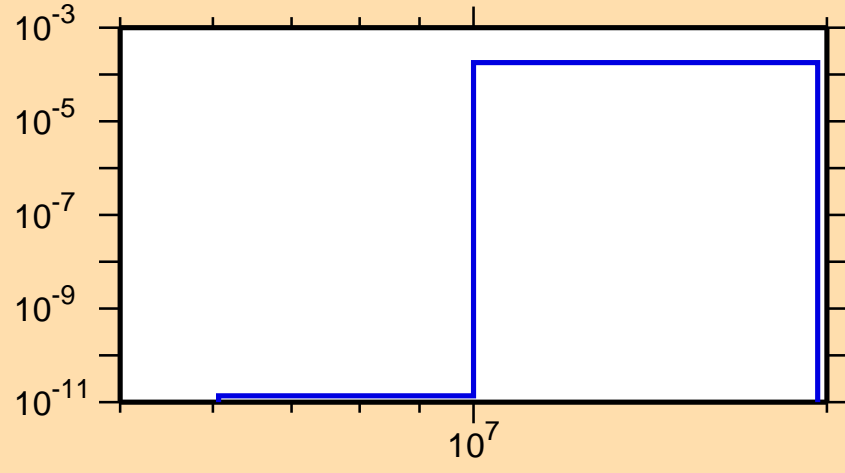
\sigma vs. E for ^{194}\text{Ir}(n,np)
