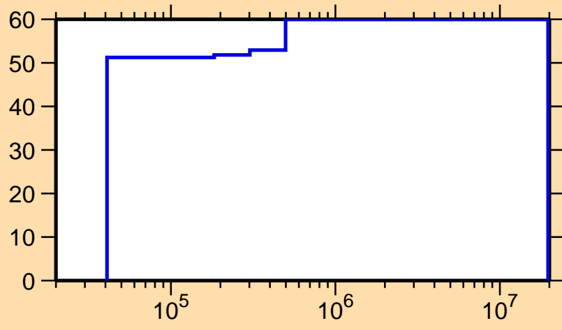
\Delta\sigma/\sigma vs. E for ^{194}\text{Ir}(n,n_1)
