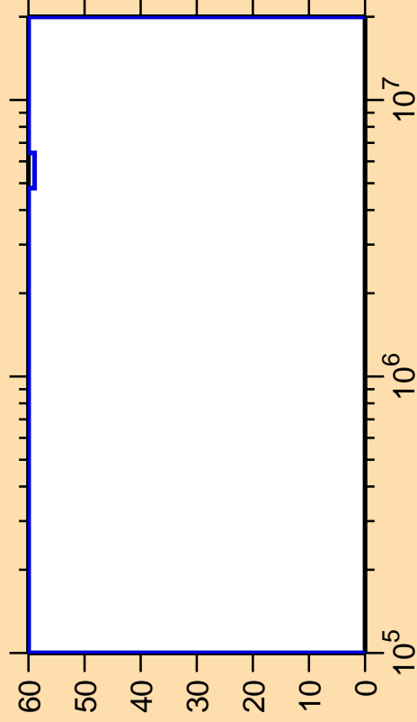
\Delta\sigma/\sigma vs. E for ^{194}\text{Ir}(n,n_4)
