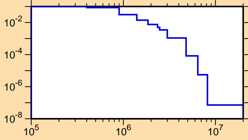
\sigma vs. E for ^{194}\text{Ir}(n,n_4)
