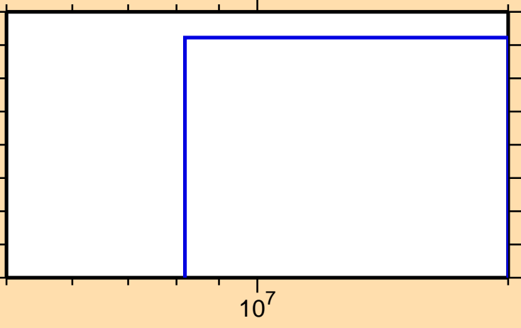
\sigma vs. E for ^{194}\text{Ir}(n,np)
