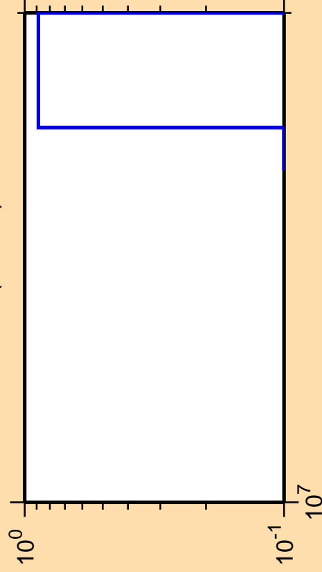
\Delta\sigma/\sigma vs. E for ^{194}\text{Ir}(n,3n\alpha)
